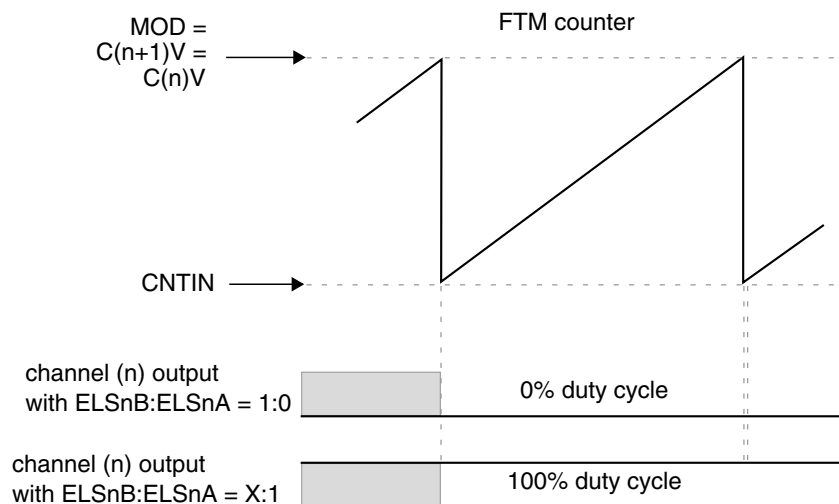
Figure 39-238. Channel (n) output if (C(n)V = C(n+1)V = MOD)
