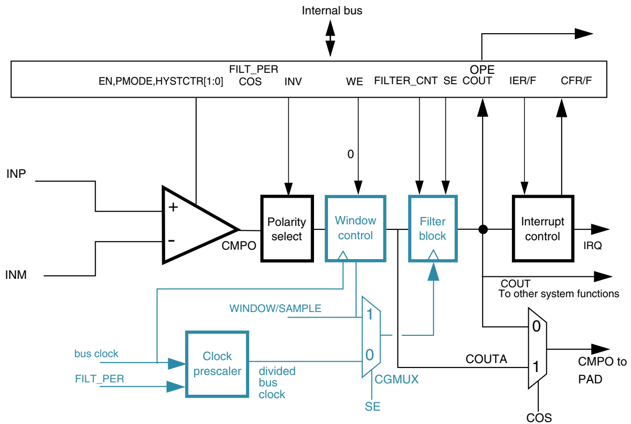
Figure 35-21. Comparator operation in Continuous mode
