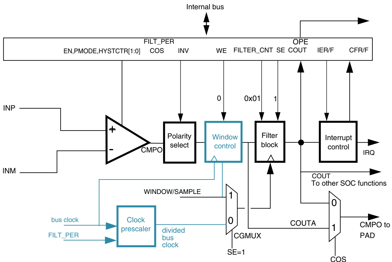
Figure 35-22. Sampled, Non-Filtered (# 3A): sampling point externally driven
