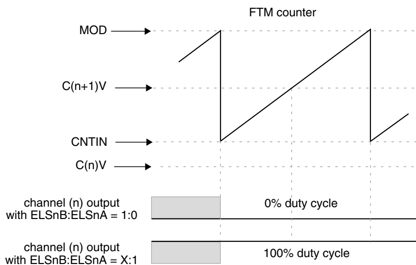
Figure 39-240. Channel (n) output if (C(n)V < CNTIN) and (CNTIN < C(n+1)V < MOD)
