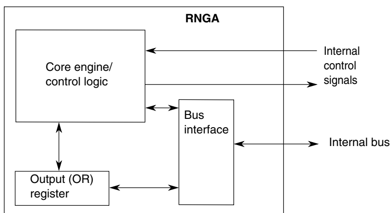
Figure 33-5. RNGA block diagram
