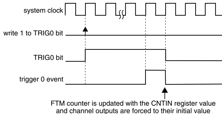
Figure 39-266. FTM counter synchronization with (SYNCMODE = 0), (HWTRIGMODE = 0), (REINIT = 1), (PWMSYNC = 1), and a hardware trigger was used
