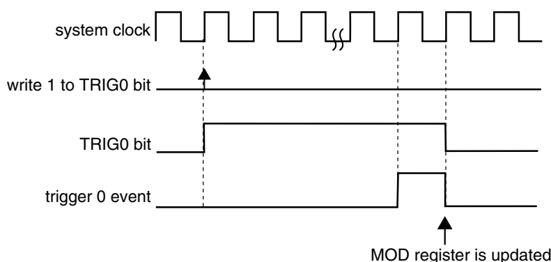
Figure 39-254. MOD synchronization with (SYNCMODE = 0), (HWTRIGMODE = 0), (PWMSYNC = 0), (REINIT = 1), and a hardware trigger was used
