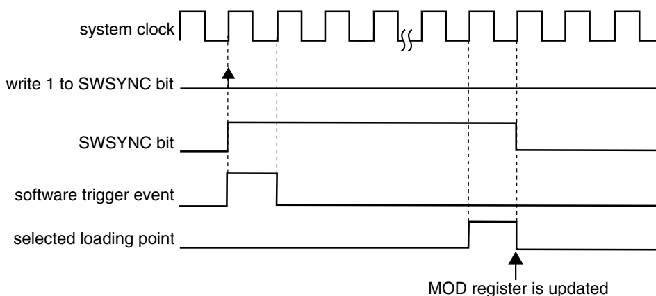
Figure 39-255. MOD synchronization with (SYNCMODE = 0) and (PWMSYNC = 1)
