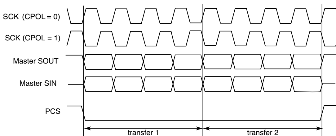
Figure 45-77. Continuous SCK timing diagram (CONT=1)
