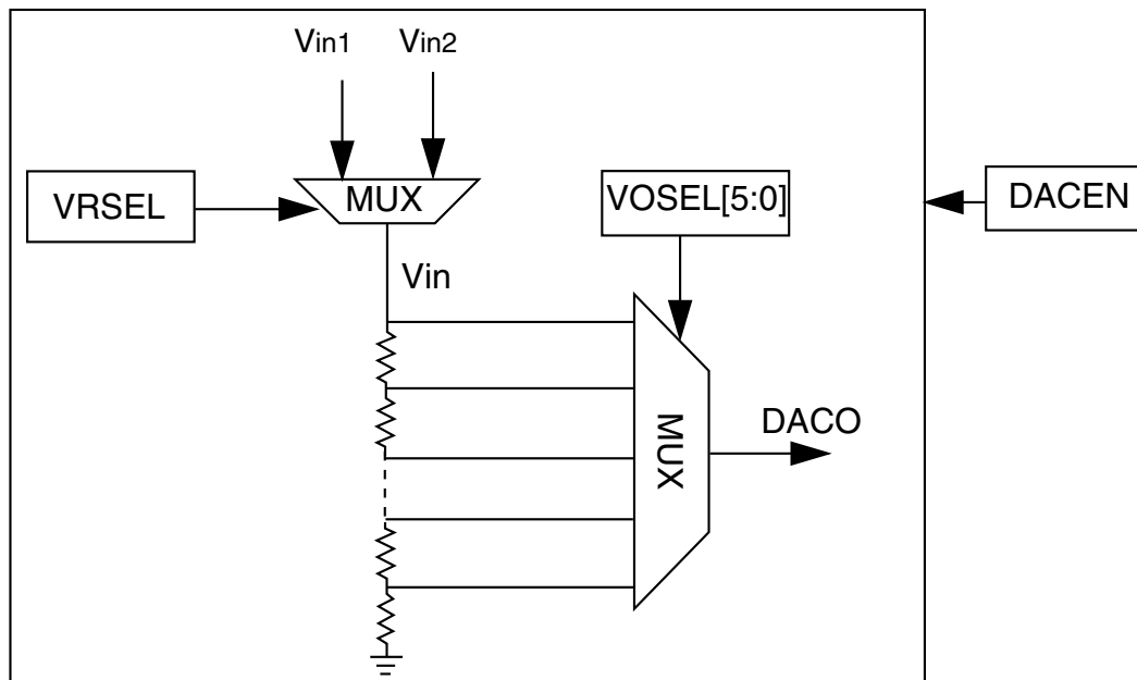
Figure 35-30. 6-bit DAC block diagram
