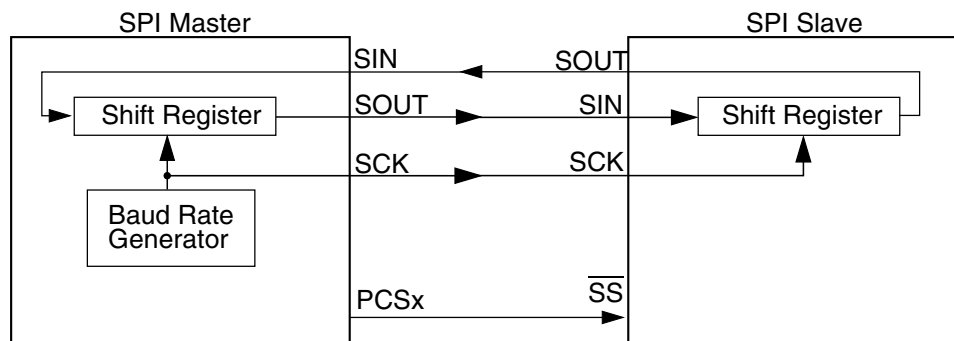
Figure 45-69. Serial protocol overview
