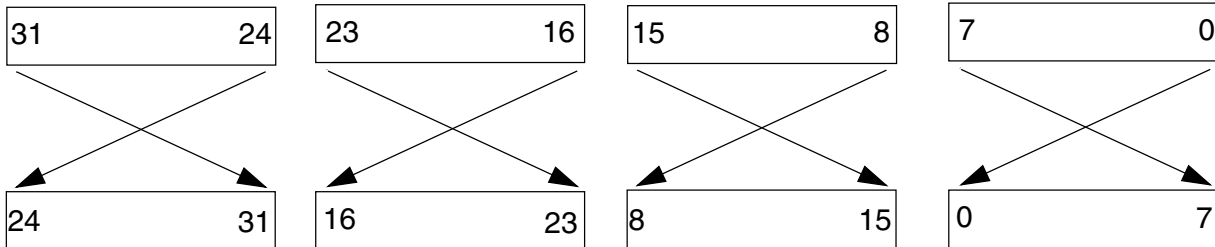
Figure 32-5. Transpose type 01
