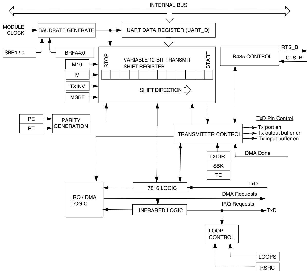
Figure 47-153. Transmitter Block Diagram
