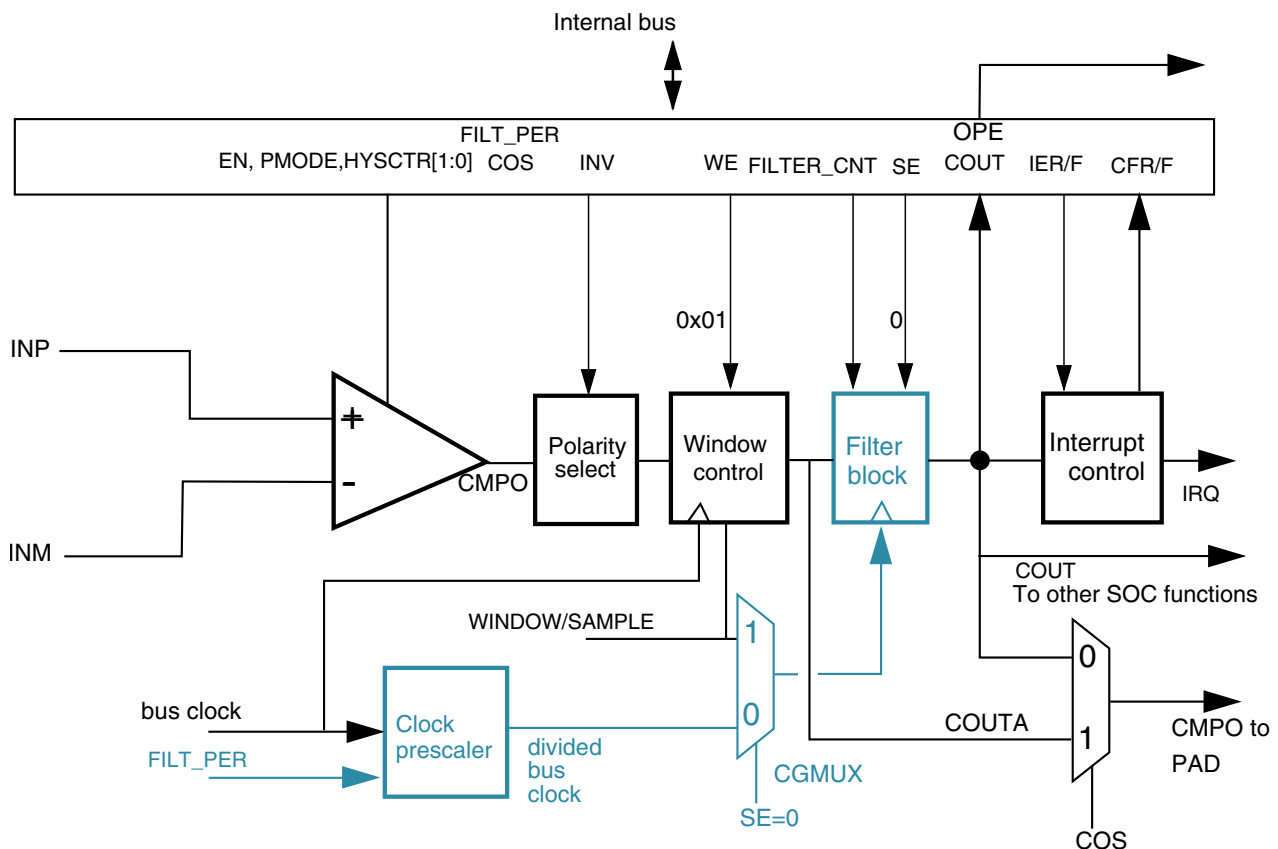
Figure 35-27. Windowed mode
