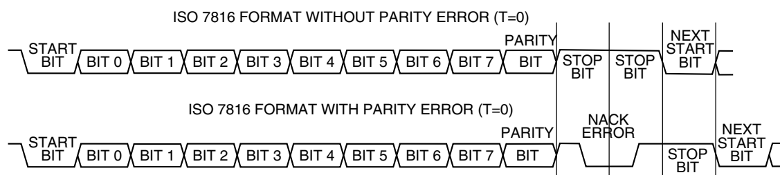
Figure 47-178. ISO-7816 T = 0 data format
