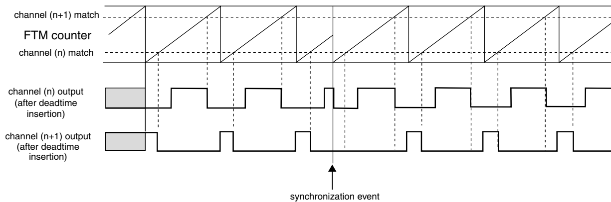
Figure 39-262. FTM counter synchronization
