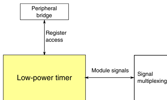
Figure 3-43. LPTMR configuration
