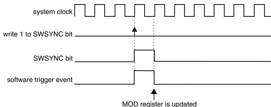
Figure 39-253. MOD synchronization with (SYNCMODE = 0), (PWMSYNC = 0), (REINIT = 1), and software trigger was used
