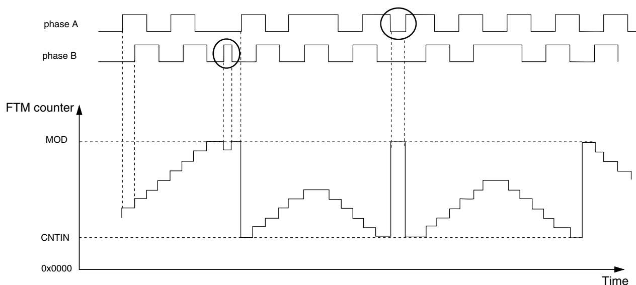
Figure 39-299. Motor position jittering near maximum and minimum count value
