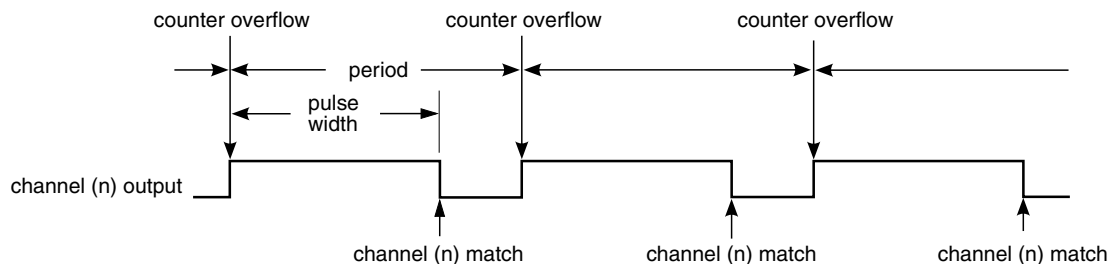
Figure 39-223. EPWM period and pulse width with ELSnB:ELSnA = 1:0
