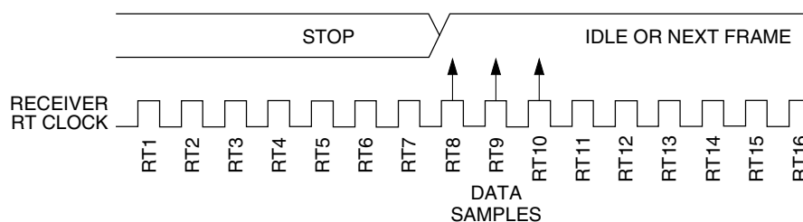
Figure 47-165. Fast data
