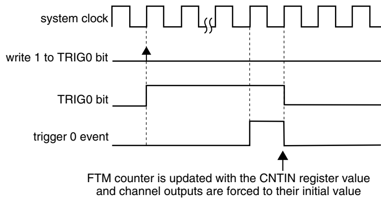
Figure 39-265. FTM counter synchronization with (SYNCMODE = 0), (HWTRIGMODE = 0), (REINIT = 1), (PWMSYNC = 0), and a hardware trigger was used
