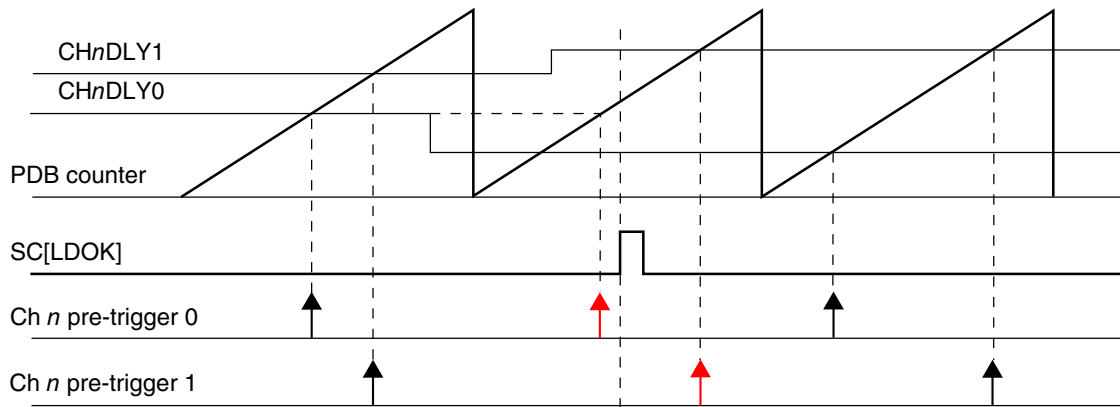
Figure 38-55. Registers update with SC[LDMOD] = 00
