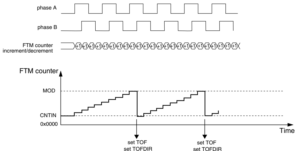
Figure 39-296. FTM Counter overflow in up counting for Quadrature Decoder mode
