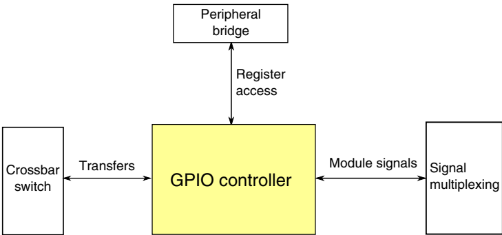
Figure 3-57. GPIO configuration
