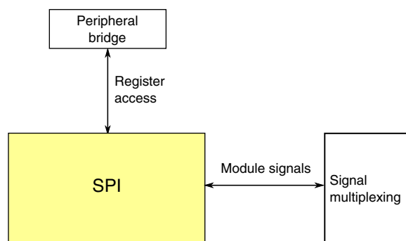
Figure 3-52. SPI configuration
