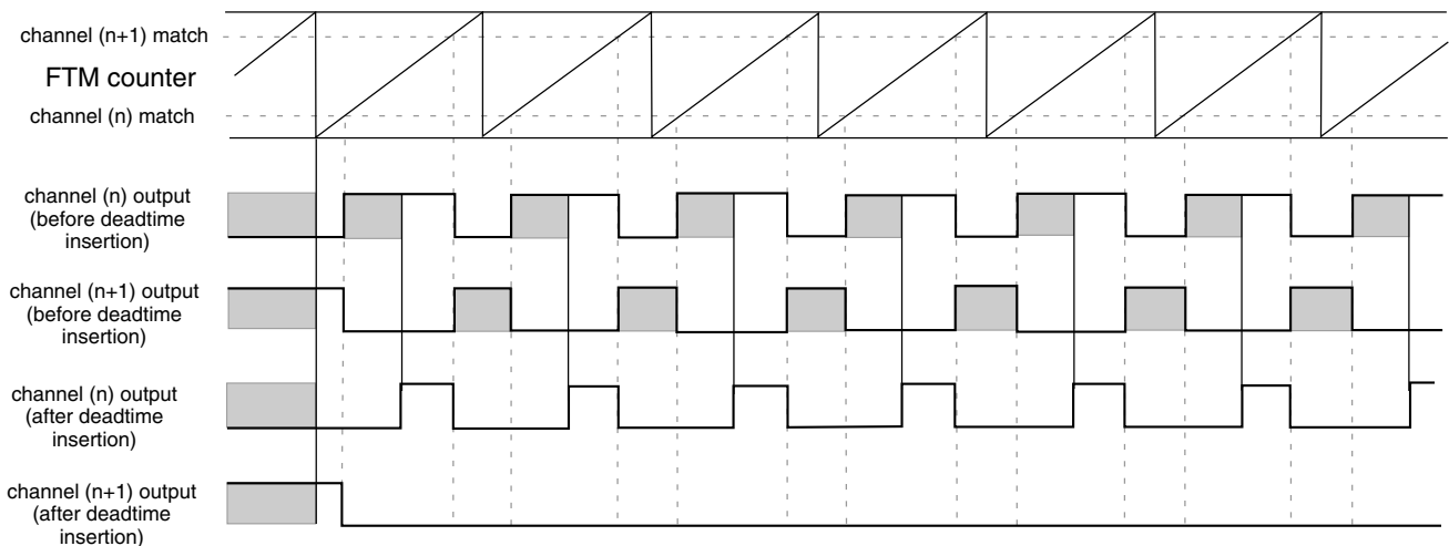
Figure 39-272. Example of the deadtime insertion (ELSnB:ELSnA = 1:0, POL(n) = 0, and POL(n+1) = 0) when the deadtime delay is comparable to channel (n+1) duty cycle
