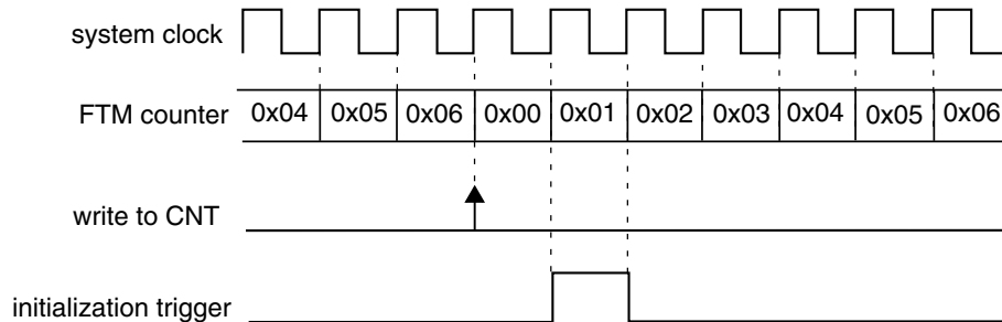
Figure 39-282. Initialization trigger is generated when there is a write to CNT register
