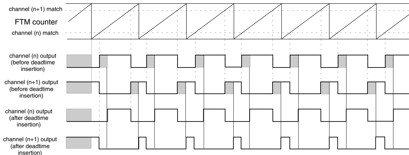
Figure 39-270. Deadtime insertion with ELSnB:ELSnA = 1:0 , POL(n) = 0 , and POL(n+1) = 0
