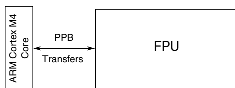
Figure 3-4. FPU configuration
