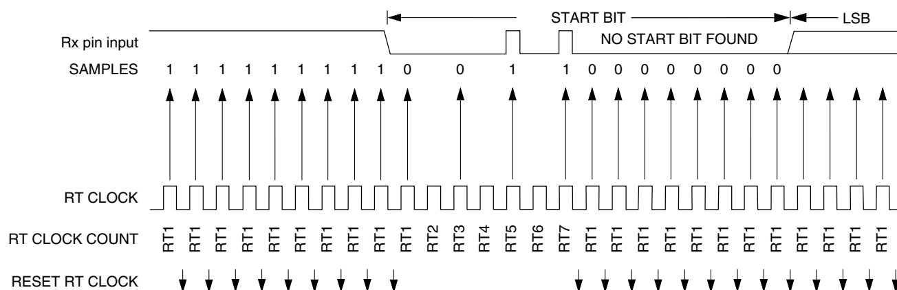
Figure 47-161. Start bit search example 5 (C7816[ISO_7816E] = 0)
