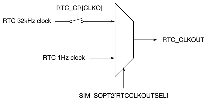
Figure 3-45. RTC_CLKOUT generation
