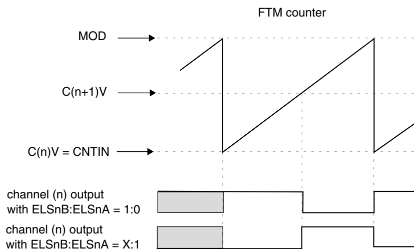
Figure 39-232. Channel (n) output if (C(n)V = CNTIN) and (CNTIN < C(n+1)V < MOD)
