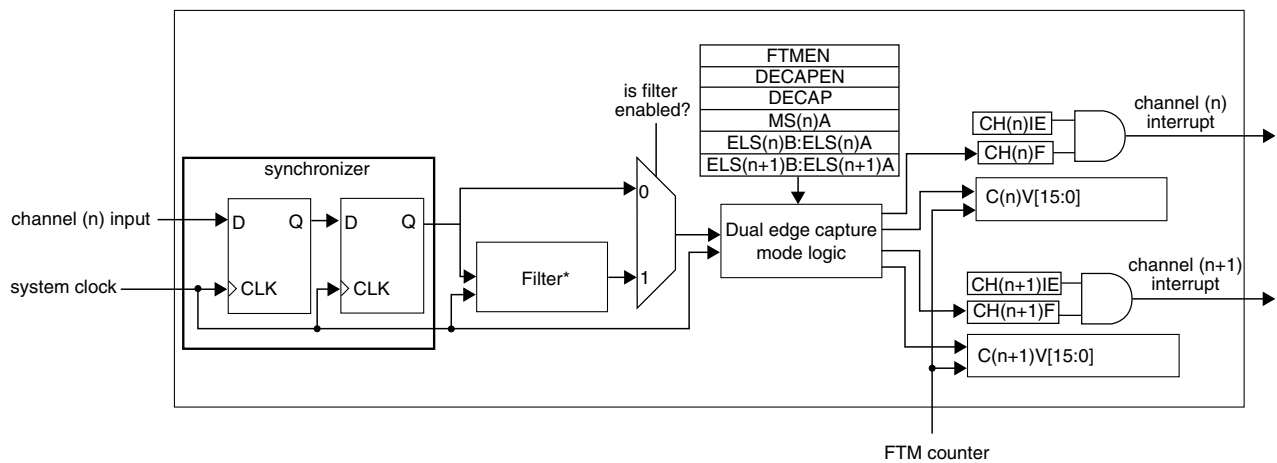
Figure 39-287. Dual Edge Capture mode block diagram
