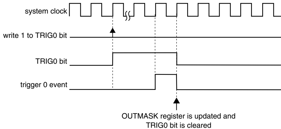
Figure 39-258. OUTMASK synchronization with (SYNCMODE = 0), (HWTRIGMODE = 0), (SYNCHOM = 1), (PWMSYNC = 0), and a hardware trigger was used
