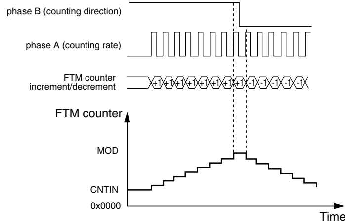
Figure 39-294. Quadrature Decoder – Count and Direction Encoding mode
