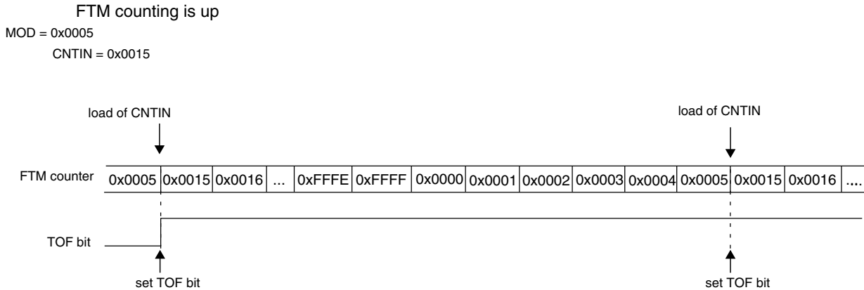
Figure 39-211. Example of up counting when the value of CNTIN is greater than the value of MOD
