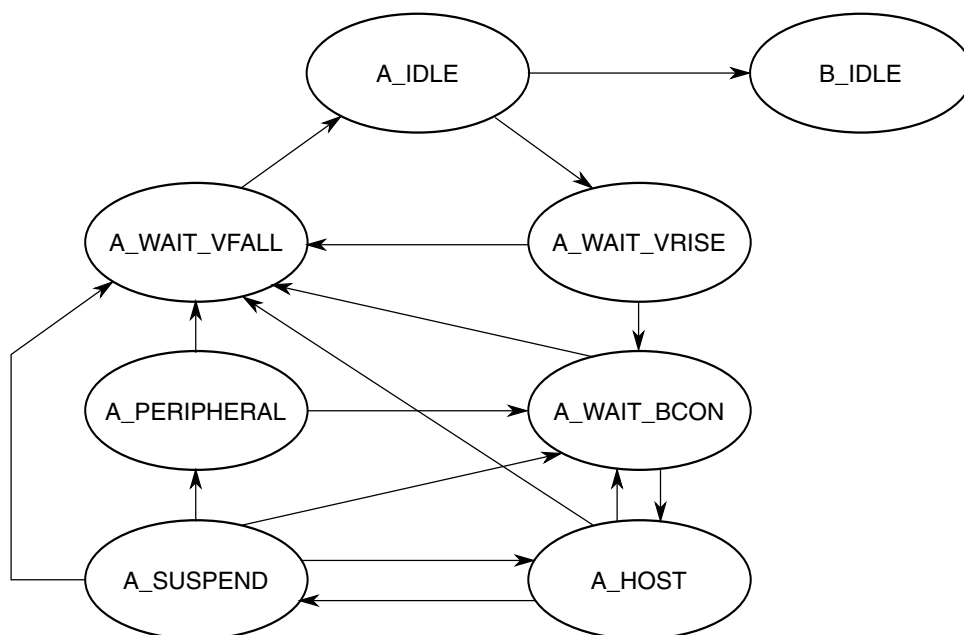
Figure 43-101. Dual role A device flow diagram
