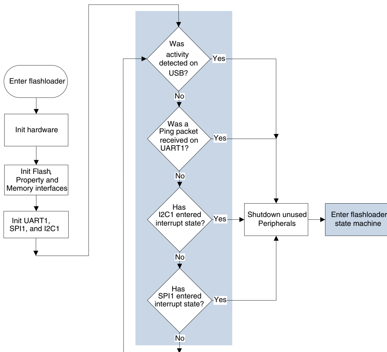
Figure 13-2. Kinetis Flashloader Start-up Flowchart
