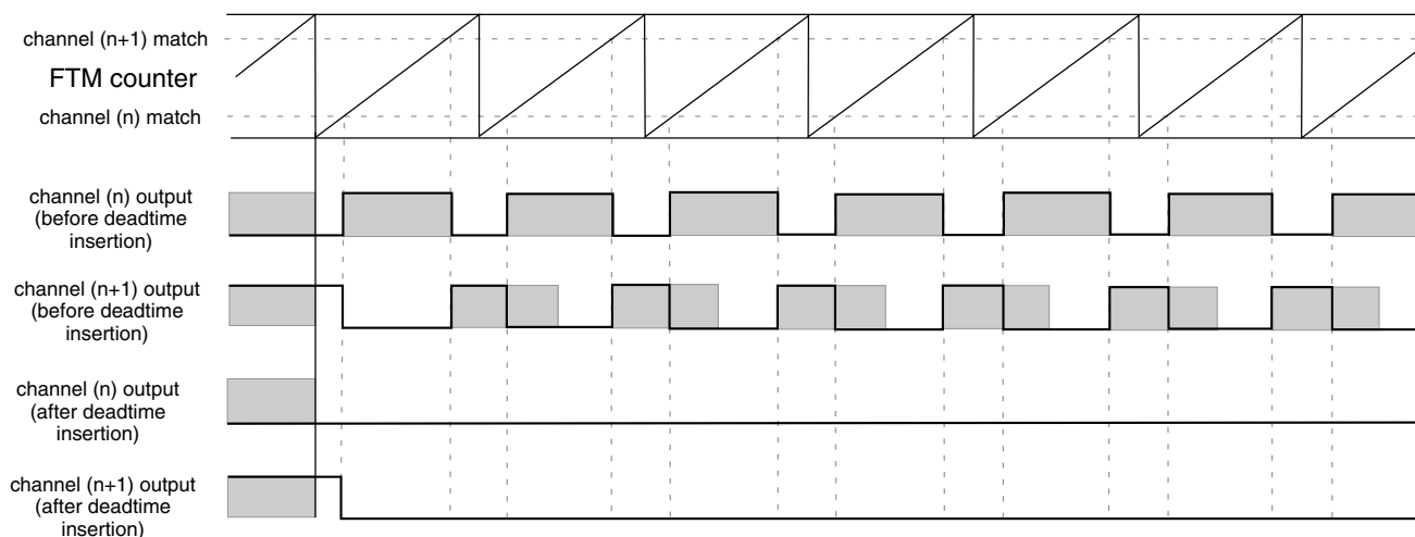
Figure 39-273. Example of the deadtime insertion ( ELSnB:ELSnA = 1:0 , POL(n) = 0 , and POL(n+1) = 0 ) when the deadtime delay is comparable to channels (n) and (n+1) duty cycle
