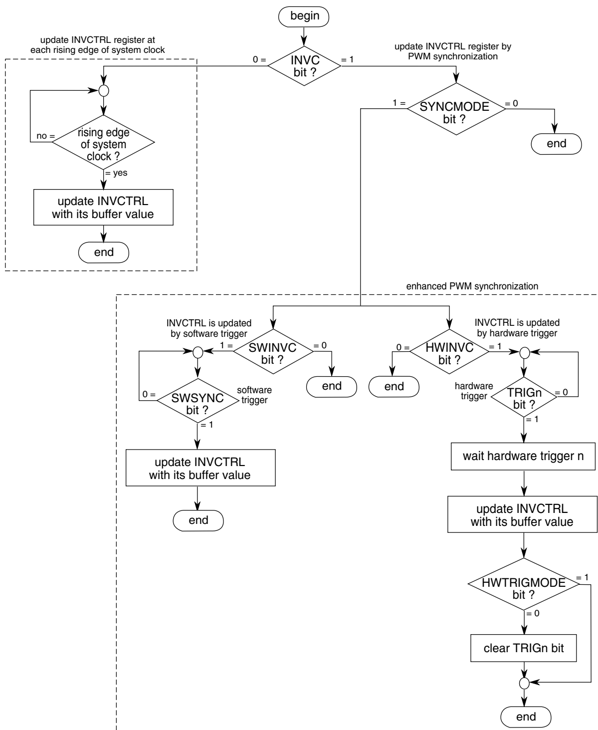
Figure 39-260. INVCTRL register synchronization flowchart
