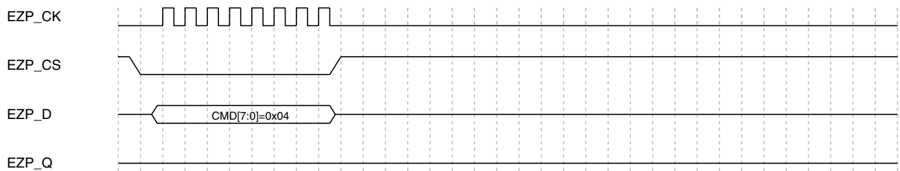
Figure 30-3. Write Disable command sequence
