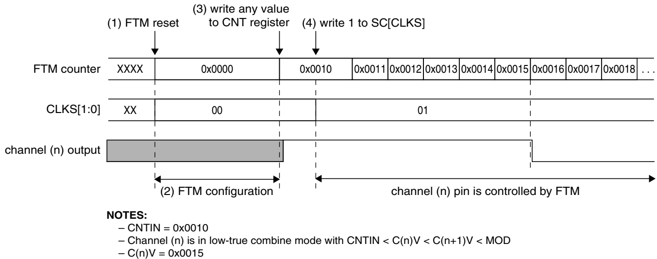
Figure 39-302. FTM behavior after reset when the channel (n) is in Combine mode
