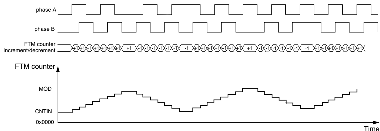
Figure 39-295. Quadrature Decoder – Phase A and Phase B Encoding mode
