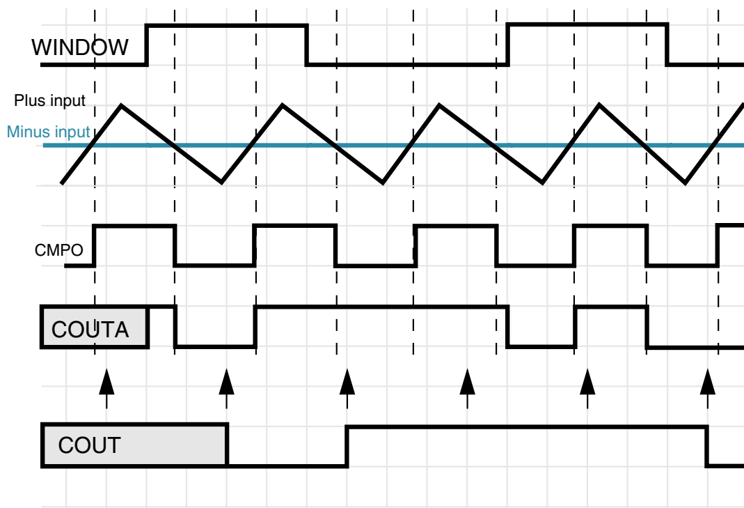
Figure 35-28. Windowed/resampled mode operation
