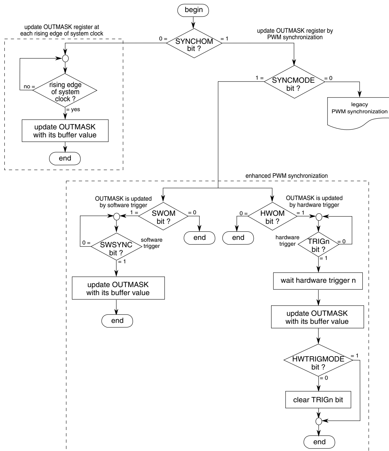
Figure 39-256. OUTMASK register synchronization flowchart
