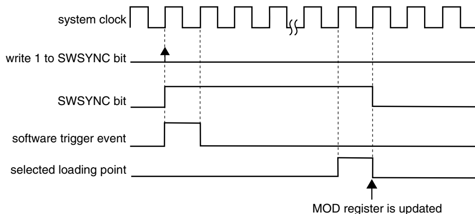
Figure 39-251. MOD synchronization with (SYNCMODE = 0), (PWMSYNC = 0), (REINIT = 0), and software trigger was used
