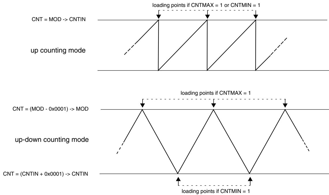
Figure 39-249. Boundary cycles and loading points
