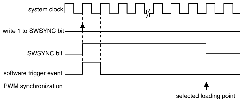
Figure 39-248. Software trigger event
