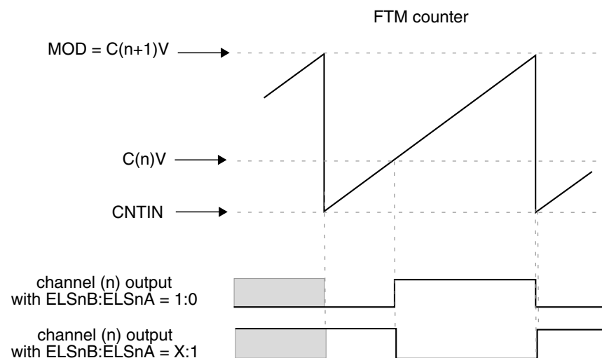
Figure 39-231. Channel (n) output if (CNTIN < C(n)V < MOD) and (C(n+1)V = MOD)
