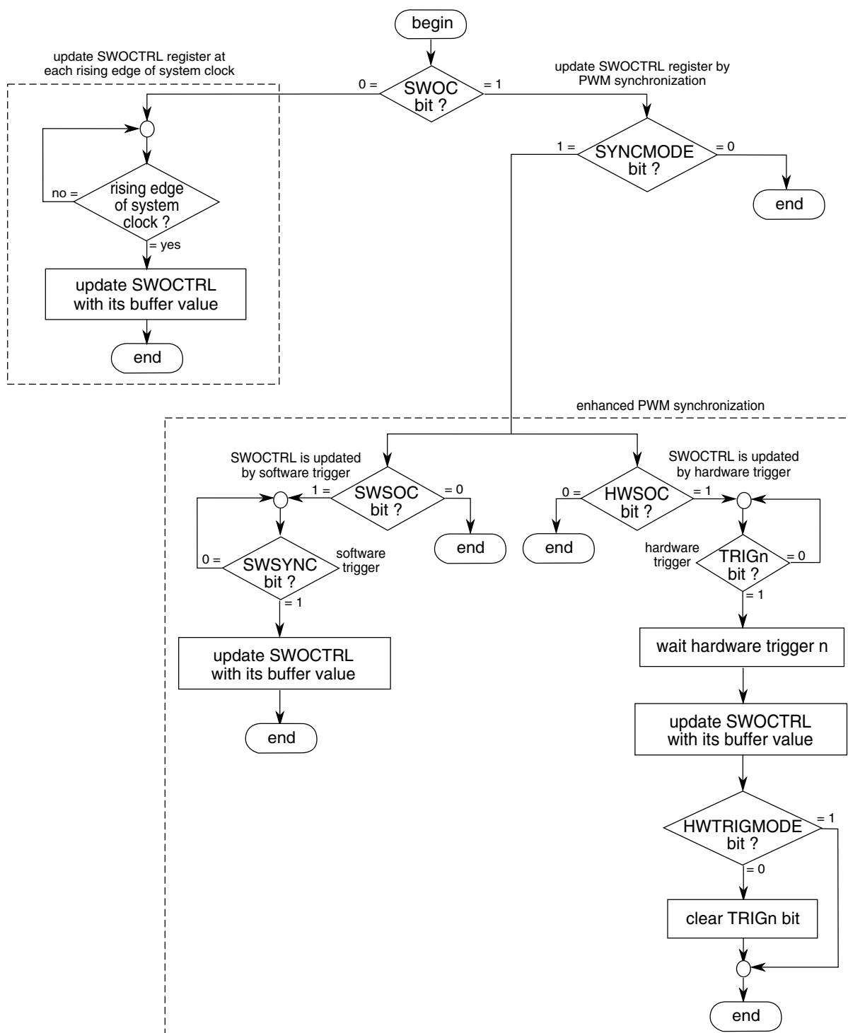
Figure 39-261. SWOCTRL register synchronization flowchart
