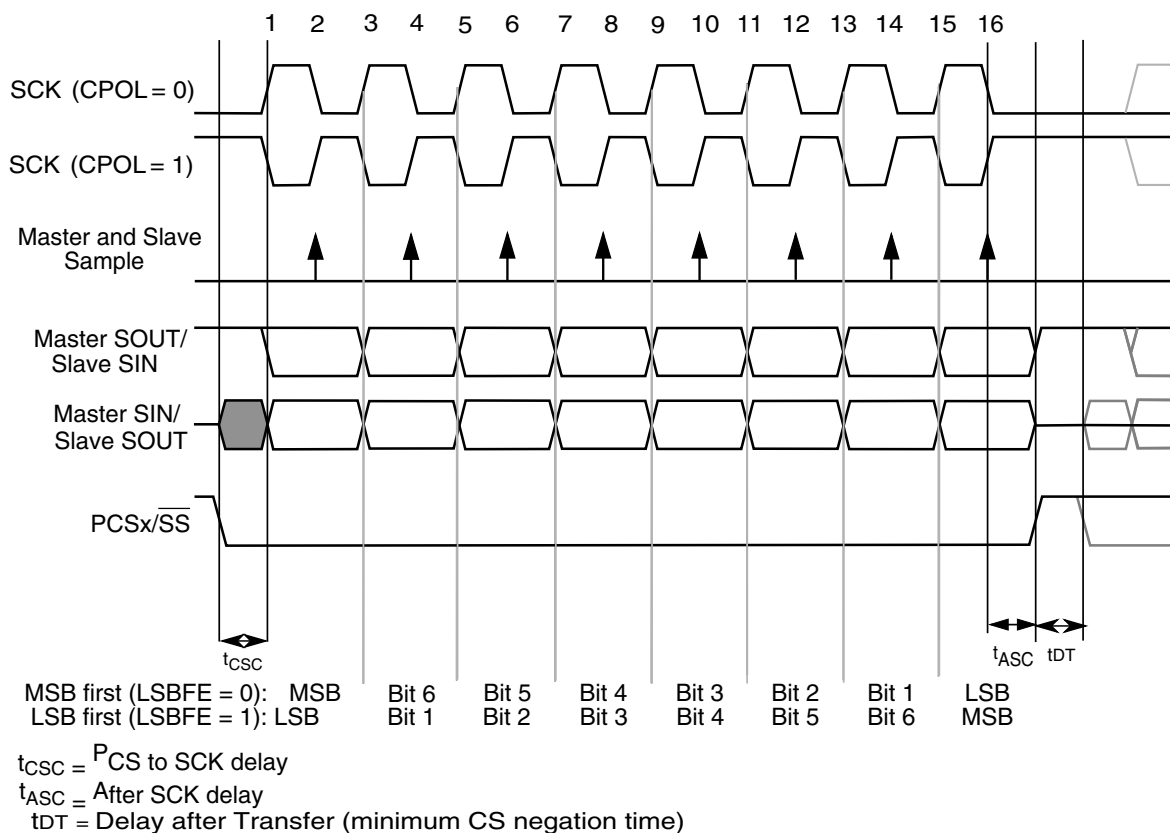
Figure 45-73. Module transfer timing diagram (MTFE=0, CPHA=1, FMSZ=8)
