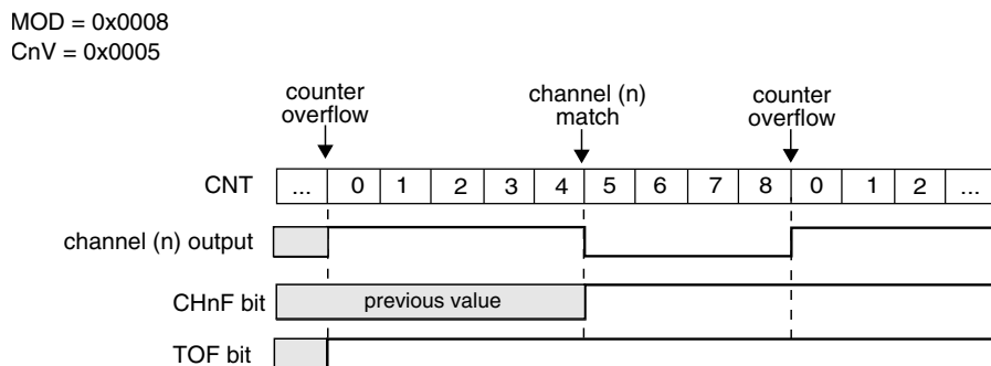
Figure 39-224. EPWM signal with ELSnB:ELSnA = 1:0
