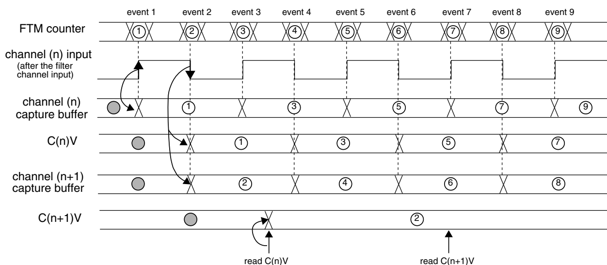
Figure 39-292. Dual Edge Capture mode read coherency mechanism
