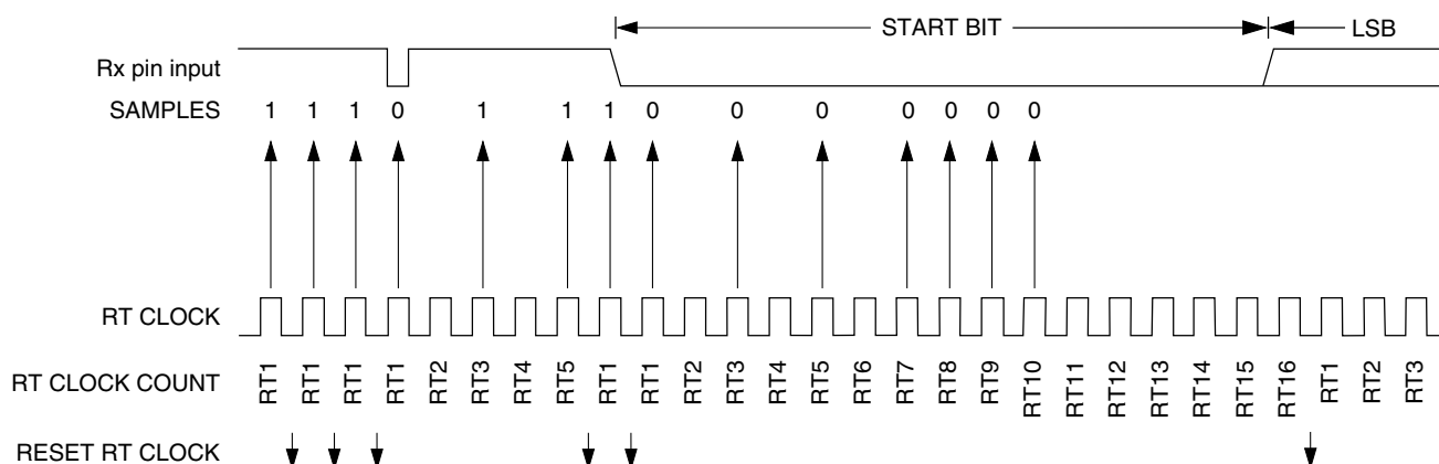
Figure 47-157. Start bit search example 1 ( C7816[ISO\_7816E] = 0 )
