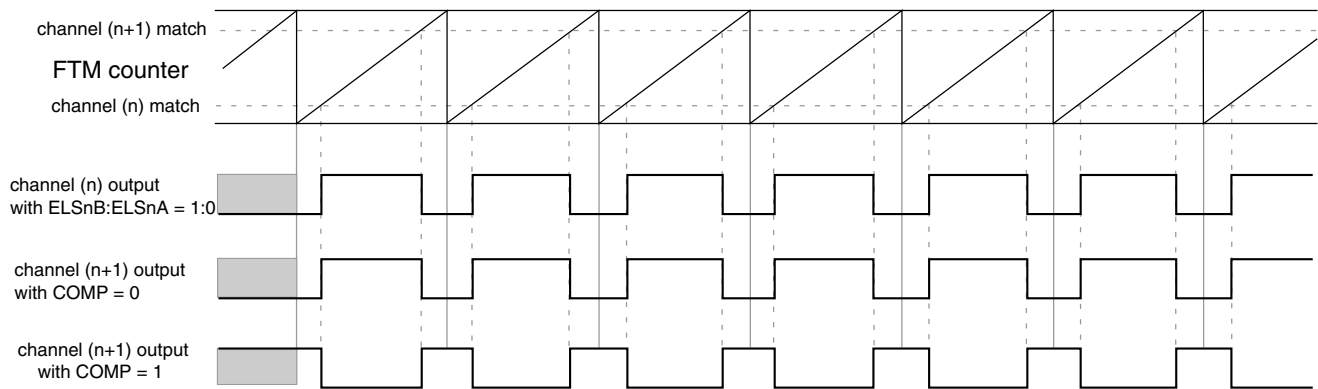
Figure 39-245. Channel (n+1) output in Complementary mode with (ELSnB:ELSnA = 1:0)
