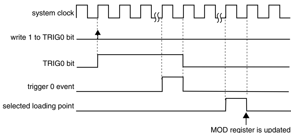
Figure 39-252. MOD synchronization with (SYNCMODE = 0), (HWTRIGMODE = 0), (PWMSYNC = 0), (REINIT = 0), and a hardware trigger was used
