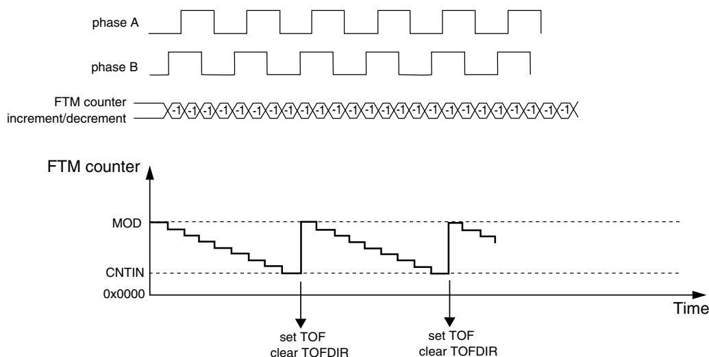
Figure 39-297. FTM counter overflow in down counting for Quadrature Decoder mode
