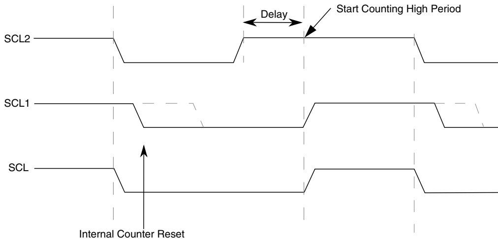
Figure 46-39. I2C clock synchronization
