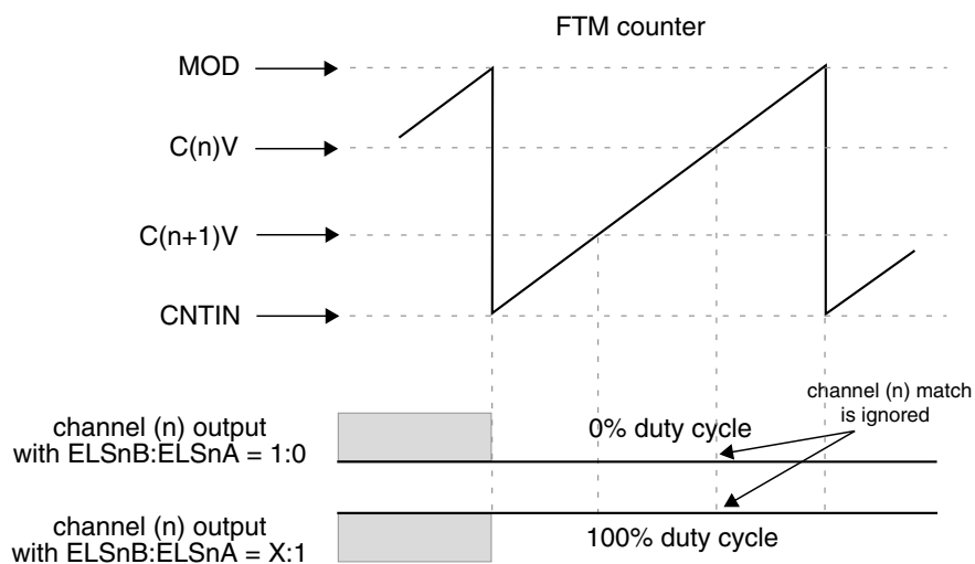
Figure 39-239. Channel (n) output if (CNTIN < C(n)V < MOD) and (CNTIN < C(n+1)V < MOD) and (C(n)V > C(n+1)V)
