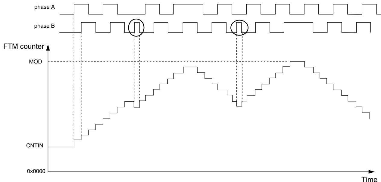
Figure 39-298. Motor position jittering in a mid count value
