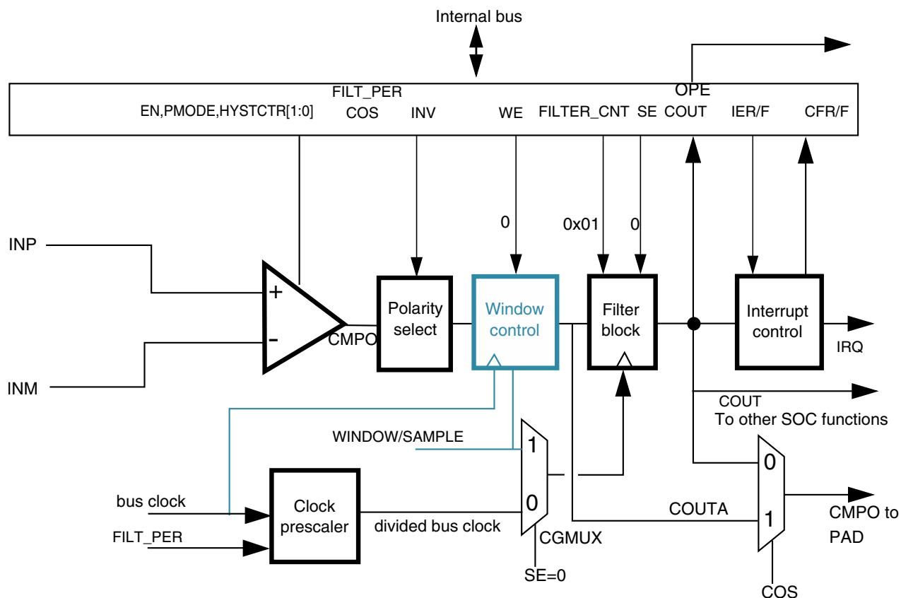
Figure 35-23. Sampled, Non-Filtered (# 3B): sampling interval internally derived
