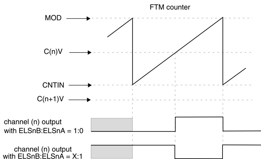
Figure 39-241. Channel (n) output if (C(n+1)V < CNTIN) and (CNTIN < C(n)V < MOD)
