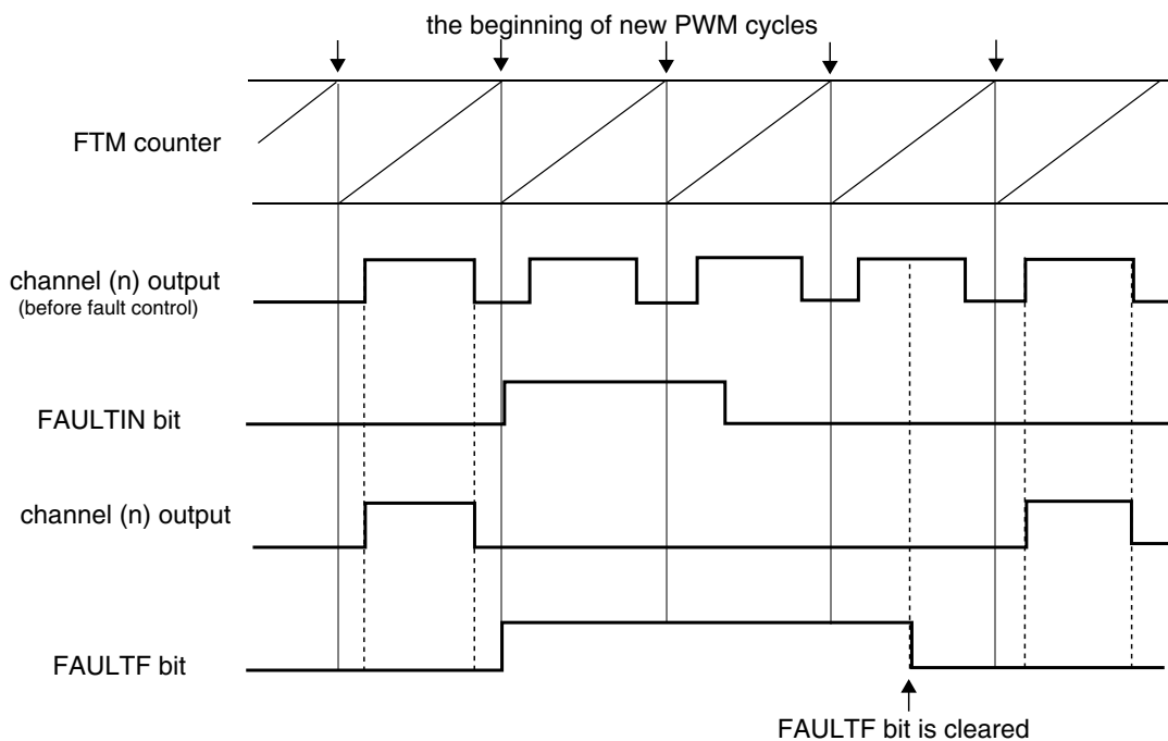
Figure 39-278. Fault control with manual fault clearing
