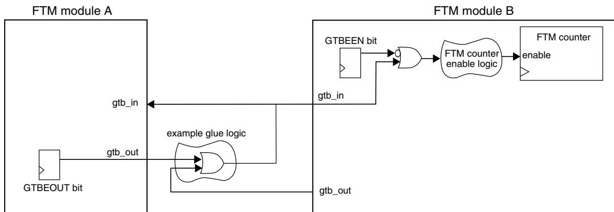
Figure 39-301. Global time base (GTB) block diagram
