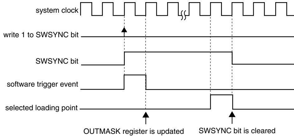
Figure 39-257. OUTMASK synchronization with (SYNCMODE = 0), (SYNCHOM = 1), (PWMSYNC = 0) and software trigger was used
