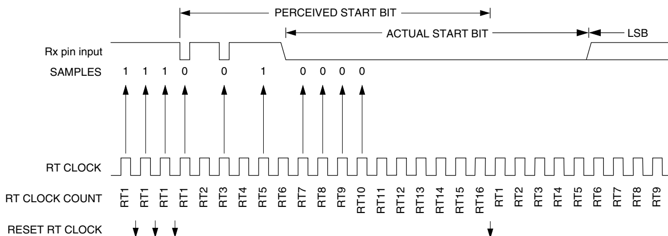
Figure 47-159. Start bit search example 3 (C7816[ISO_7816E] = 0)
