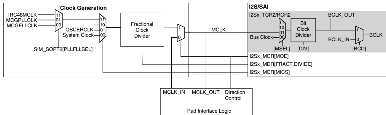
Figure 5-9. I²S/SAI clock generation
