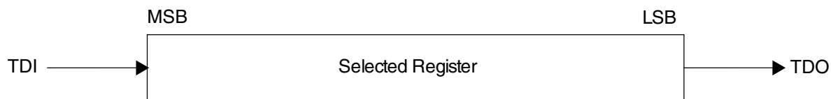
Figure 51-3. Shifting data through a register
