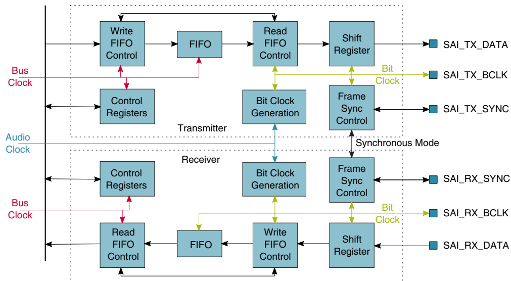
Figure 49-1. I²S/SAI block diagram
