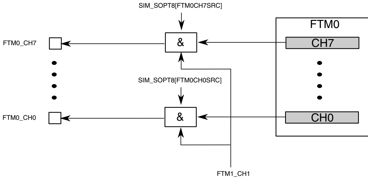
Figure 3-40. FTM Output Modulation
