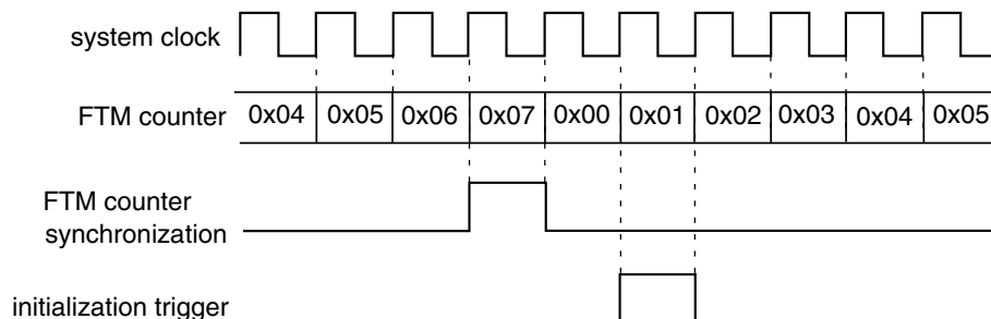
Figure 39-283. Initialization trigger is generated when there is the FTM counter synchronization
