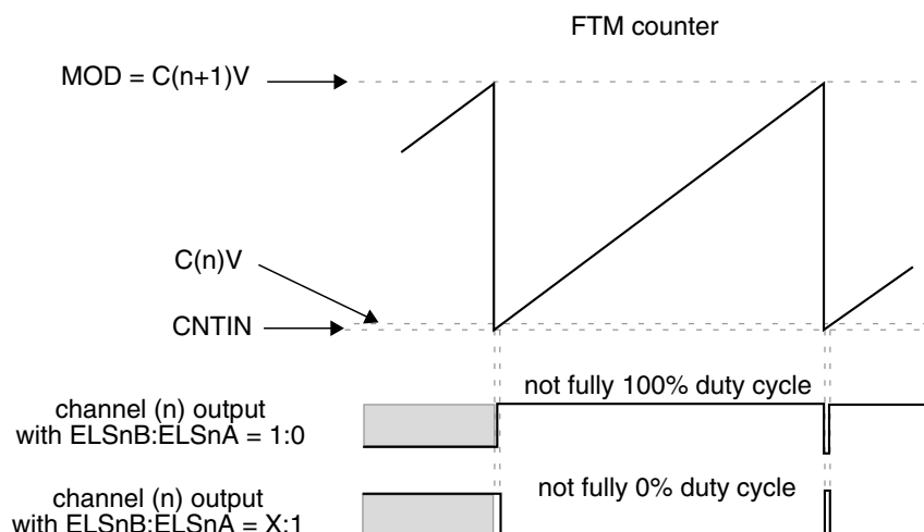
Figure 39-233. Channel (n) output if (CNTIN < C(n)V < MOD) and (C(n)V is Almost Equal to CNTIN) and (C(n+1)V = MOD)
