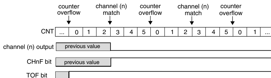
Figure 39-221. Example of the Output Compare mode when the match clears the channel output
