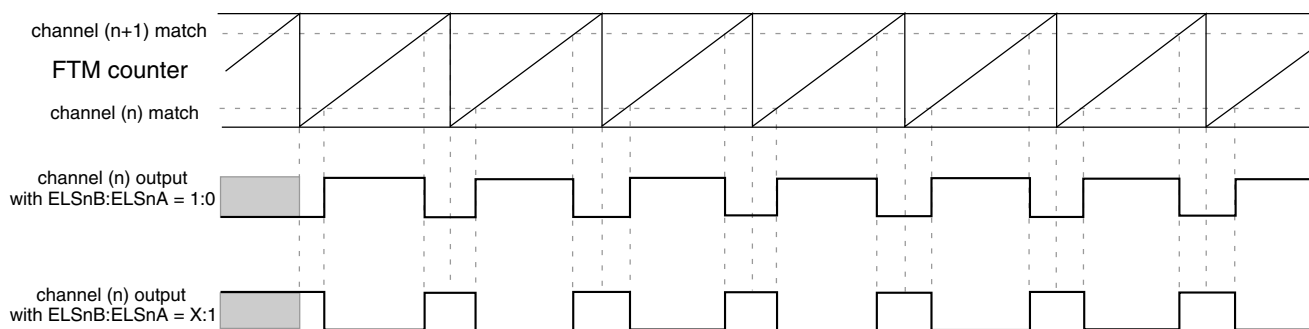
Figure 39-229. Combine mode
