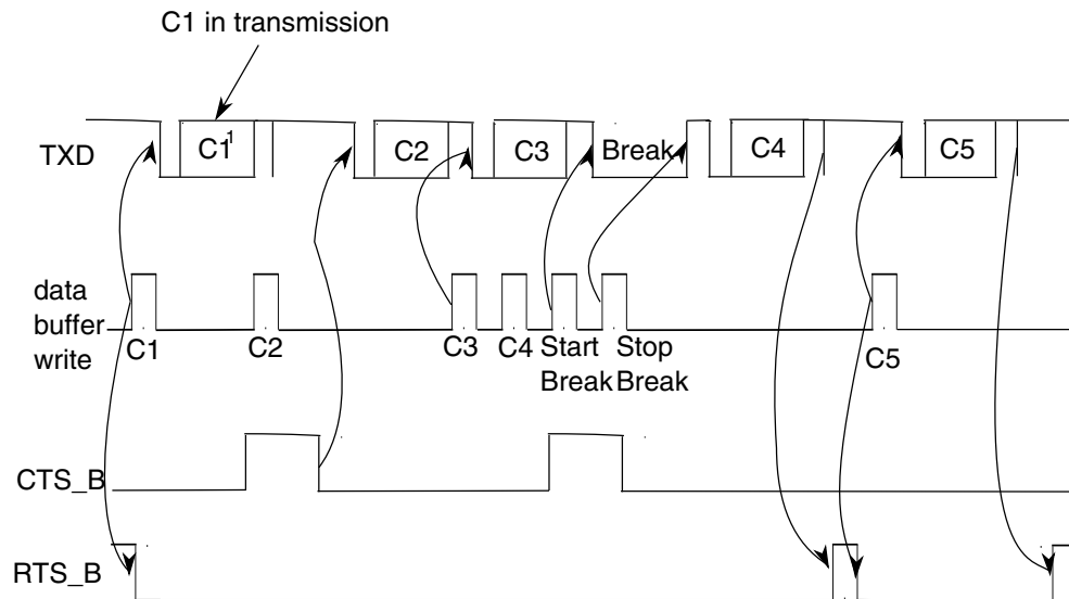
Figure 47-154. Transmitter RTS and CTS timing diagram
