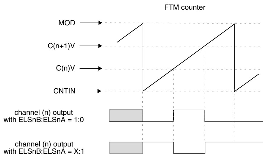
Figure 39-230. Channel (n) output if (CNTIN < C(n)V < MOD) and (CNTIN < C(n+1)V < MOD) and (C(n)V < C(n+1)V)
