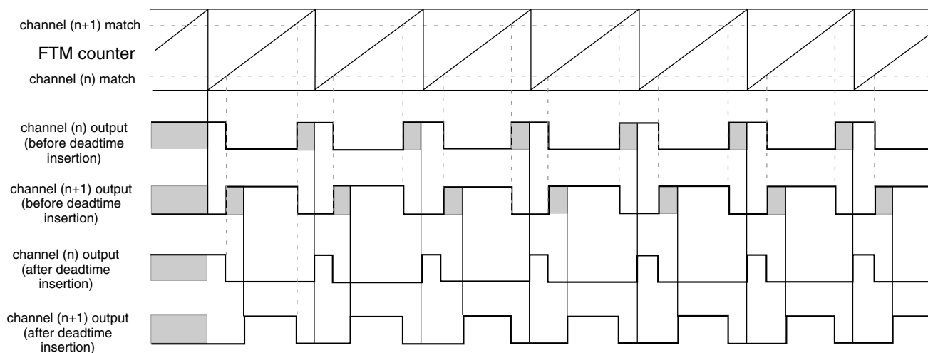
Figure 39-271. Deadtime insertion with ELSnB:ELSnA = X:1 , POL(n) = 0 , and POL(n+1) = 0
