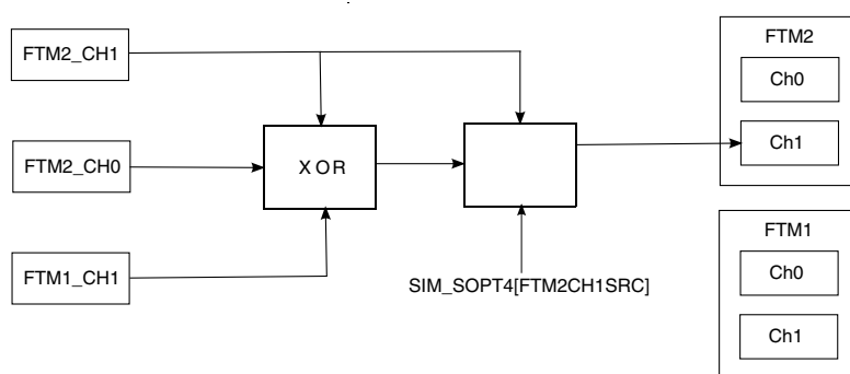
Figure 3-39. FTM Hall Sensor Configuration
