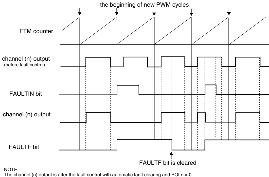
Figure 39-277. Fault control with automatic fault clearing
