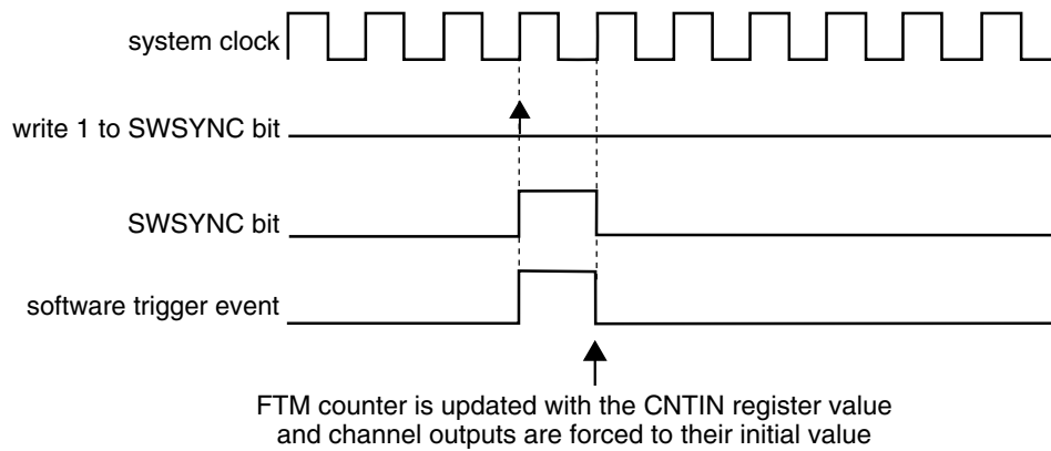
Figure 39-264. FTM counter synchronization with (SYNCMODE = 0), (REINIT = 1), (PWMSYNC = 0), and software trigger was used
