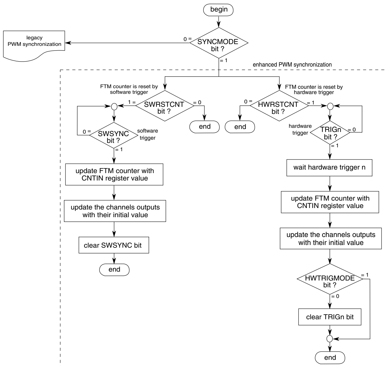
Figure 39-263. FTM counter synchronization flowchart
