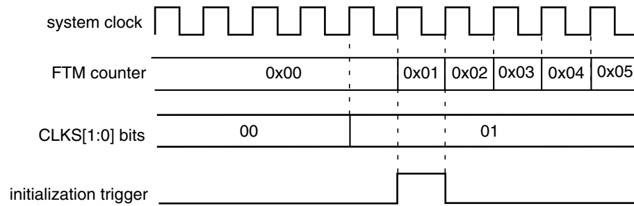
Figure 39-284. Initialization trigger is generated if (CNT = CNTIN), (CLKS[1:0] = 0:0), and a value different from zero is written to CLKS[1:0] bits
