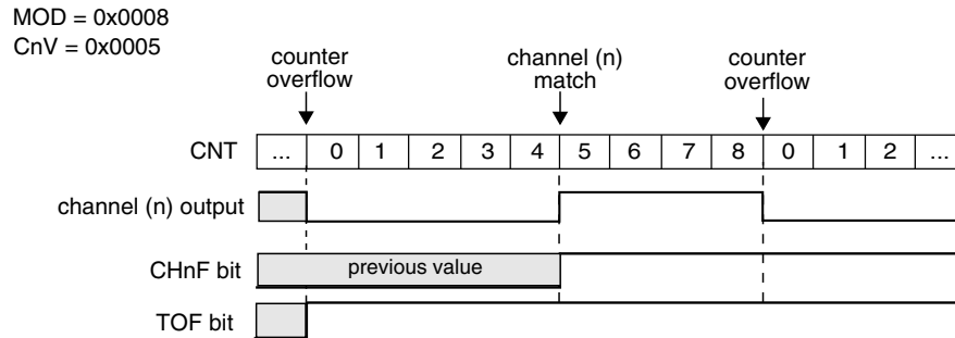
Figure 39-225. EPWM signal with ELSnB:ELSnA = X:1
