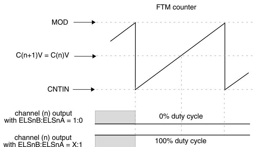
Figure 39-236. Channel (n) output if (CNTIN < C(n)V < MOD) and (CNTIN < C(n+1)V < MOD) and (C(n)V = C(n+1)V)
