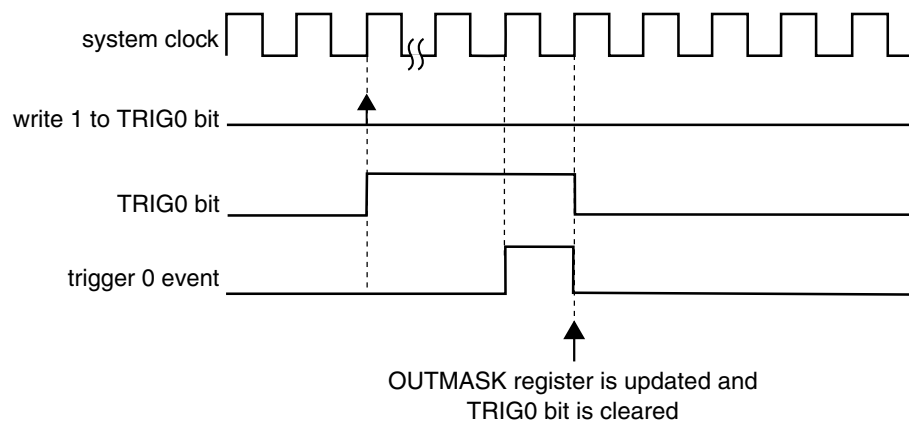
Figure 39-259. OUTMASK synchronization with (SYNCMODE = 0), (HWTRIGMODE = 0), (SYNCHOM = 1), (PWMSYNC = 1), and a hardware trigger was used
