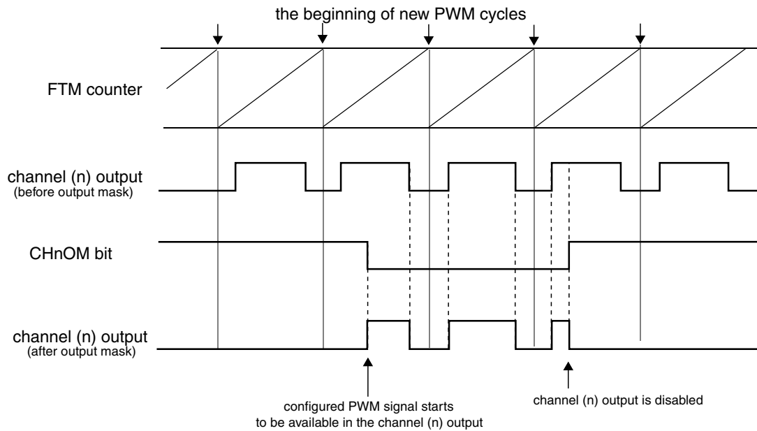
Figure 39-274. Output mask with POLn = 0
