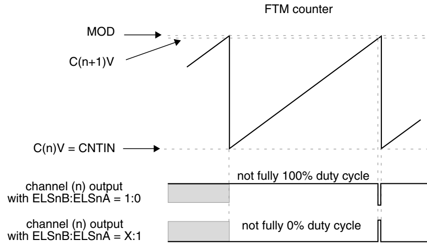
Figure 39-234. Channel (n) output if C(n)V = \text{CNTIN} and \text{CNTIN} < C(n+1)V < \text{MOD} and C(n+1)V is Almost Equal to MOD)
