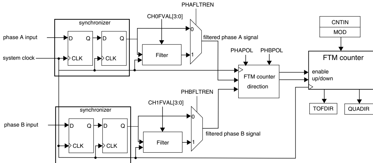
Figure 39-293. Quadrature Decoder block diagram
