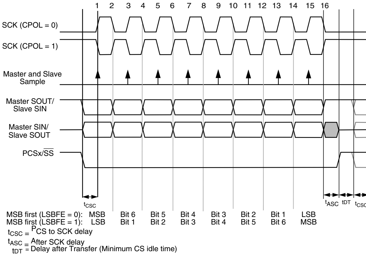
Figure 45-72. Module transfer timing diagram (MTFE=0, CPHA=0, FMSZ=8)
