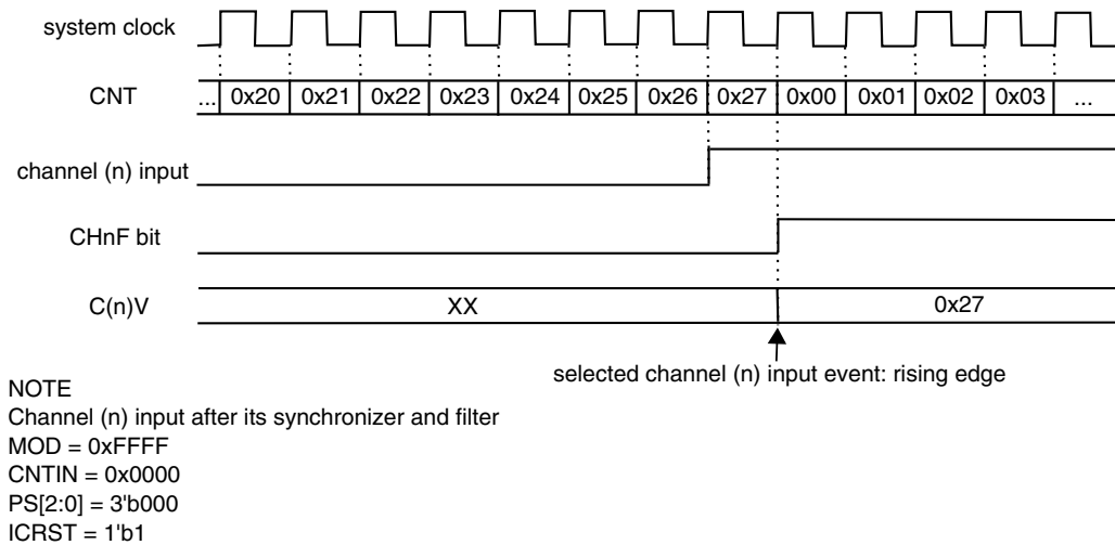
Figure 39-219. Example of the Input Capture mode with ICRST = 1
