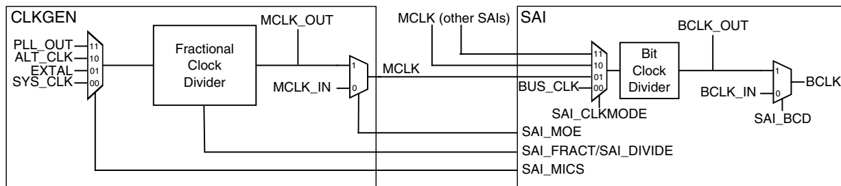
Figure 49-50. SAI master clock generation
