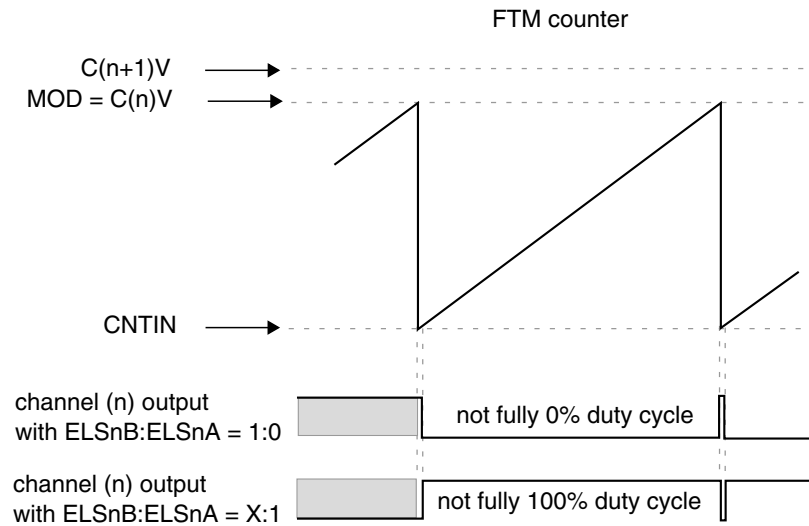
Figure 39-244. Channel (n) output if (C(n+1)V > MOD) and (CNTIN < C(n)V = MOD)
