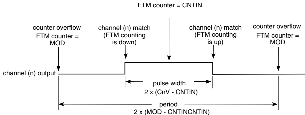
Figure 39-226. CPWM period and pulse width with ELSnB:ELSnA = 1:0
