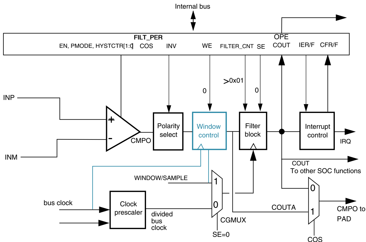
Figure 35-25. Sampled, Filtered (# 4B): sampling point internally derived
