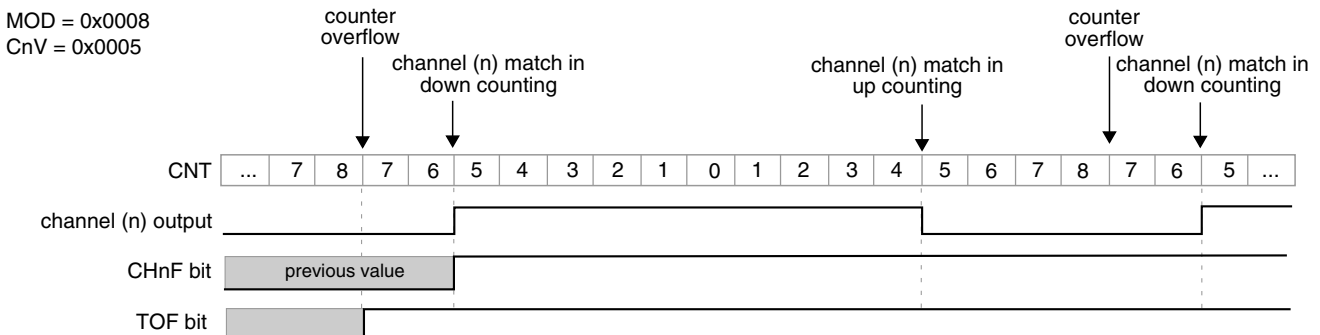
Figure 39-227. CPWM signal with ELSnB:ELSnA = 1:0
