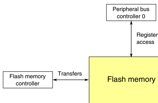
Figure 3-19. Flash memory configuration
