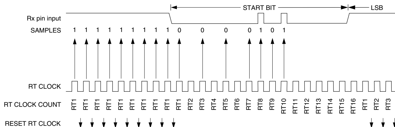
Figure 47-162. Start bit search example 6
