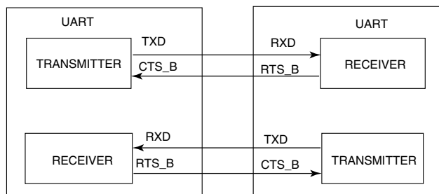
Figure 47-180. Ready-to-receive
