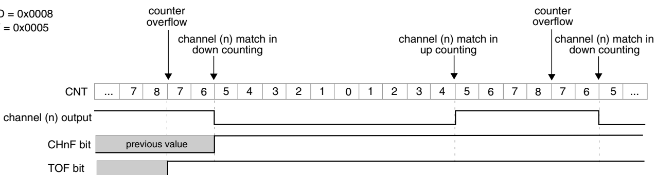
Figure 39-228. CPWM signal with ELSnB:ELSnA = X:1
