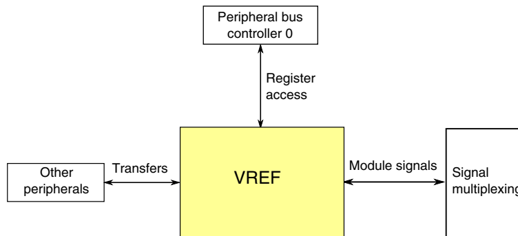
Figure 3-35. VREF configuration
