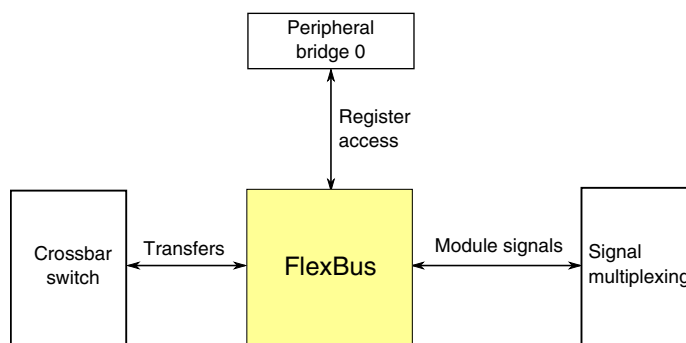
Figure 3-26. FlexBus configuration
