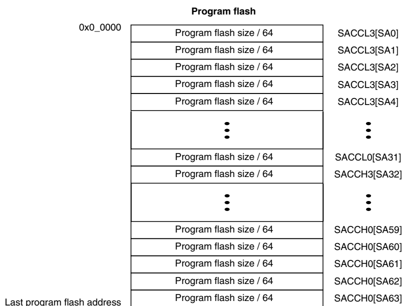
Figure 29-46. Program flash access control (256KB or 512KB of program flash)
