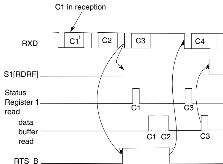
Figure 47-163. Receiver hardware flow control timing diagram
