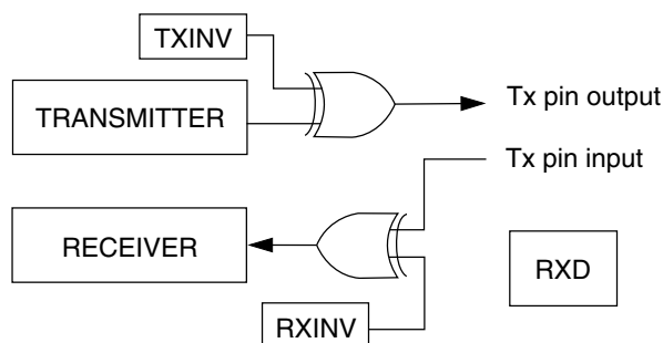
Figure 47-176. Single-wire operation (C1[LOOPS] = 1, C1[RSRC] = 1)
