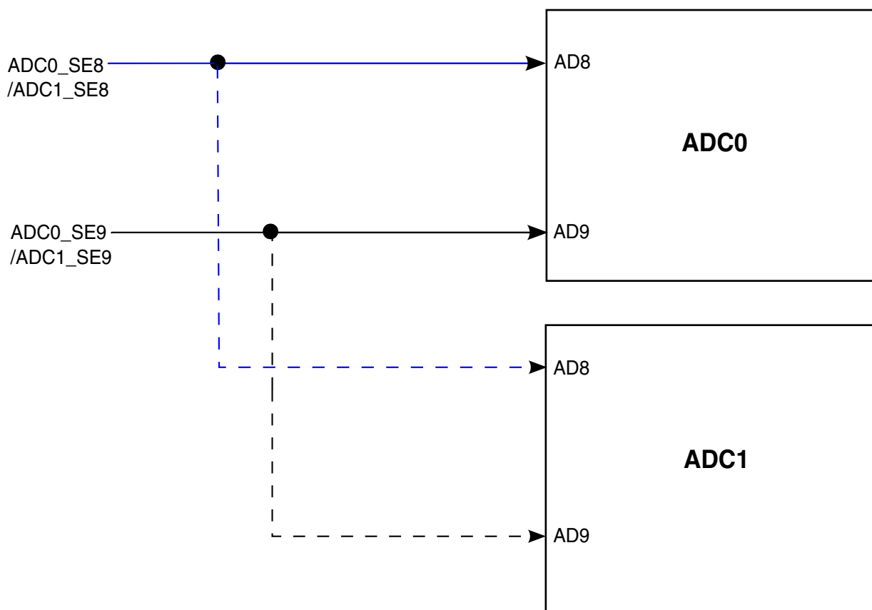
Figure 3-32. ADC hardware interleaved channels integration
