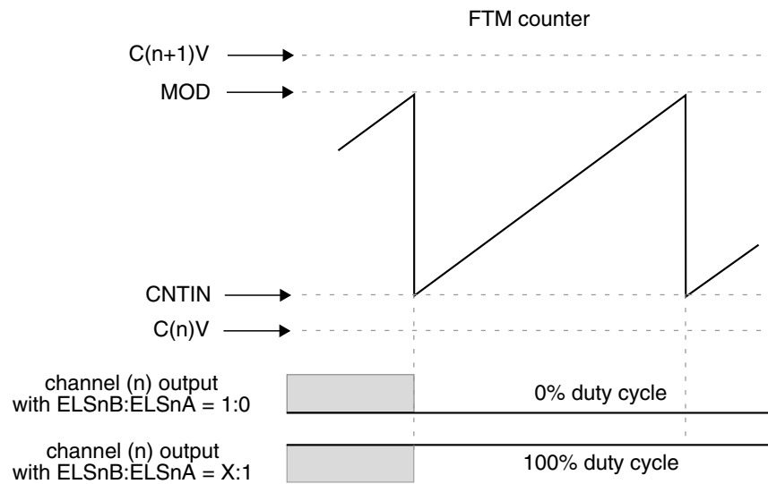
Figure 39-235. Channel (n) output if C(n)V and C(n+1)V are not between \text{CNTIN} and \text{MOD}
