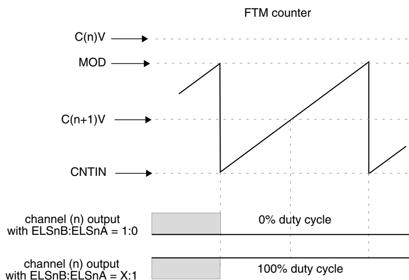
Figure 39-242. Channel (n) output if (C(n)V > MOD) and (CNTIN < C(n+1)V < MOD)
