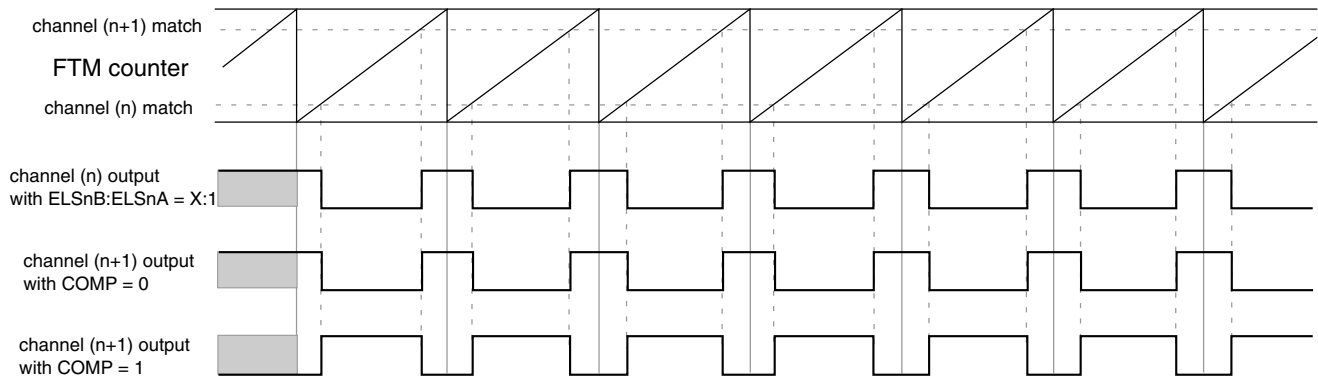
Figure 39-246. Channel (n+1) output in Complementary mode with (ELSnB:ELSnA = X:1)
