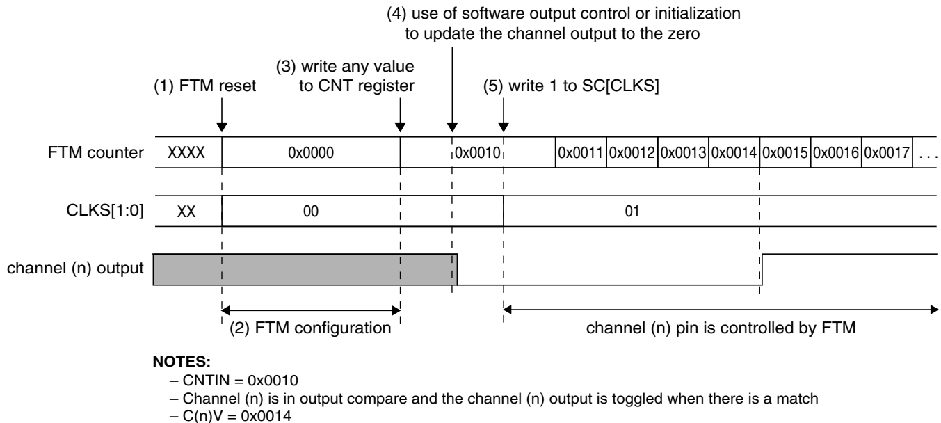
Figure 39-303. FTM behavior after reset when the channel (n) is in Output Compare mode
