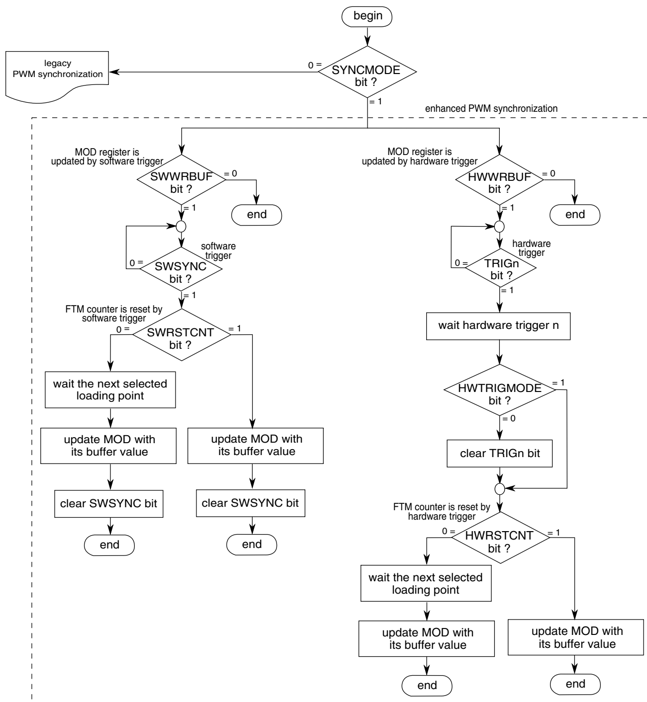
Figure 39-250. MOD register synchronization flowchart
