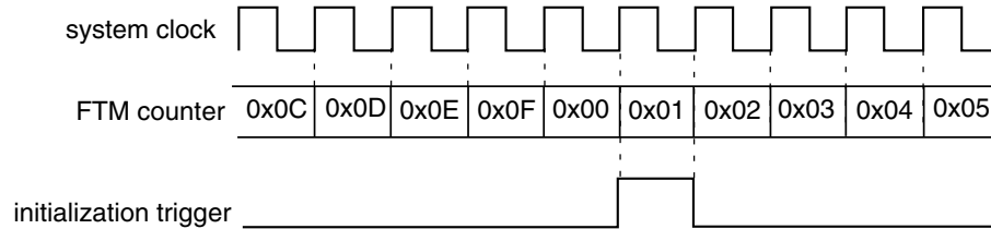
Figure 39-281. Initialization trigger is generated when the FTM counting achieves the CNTIN register value
