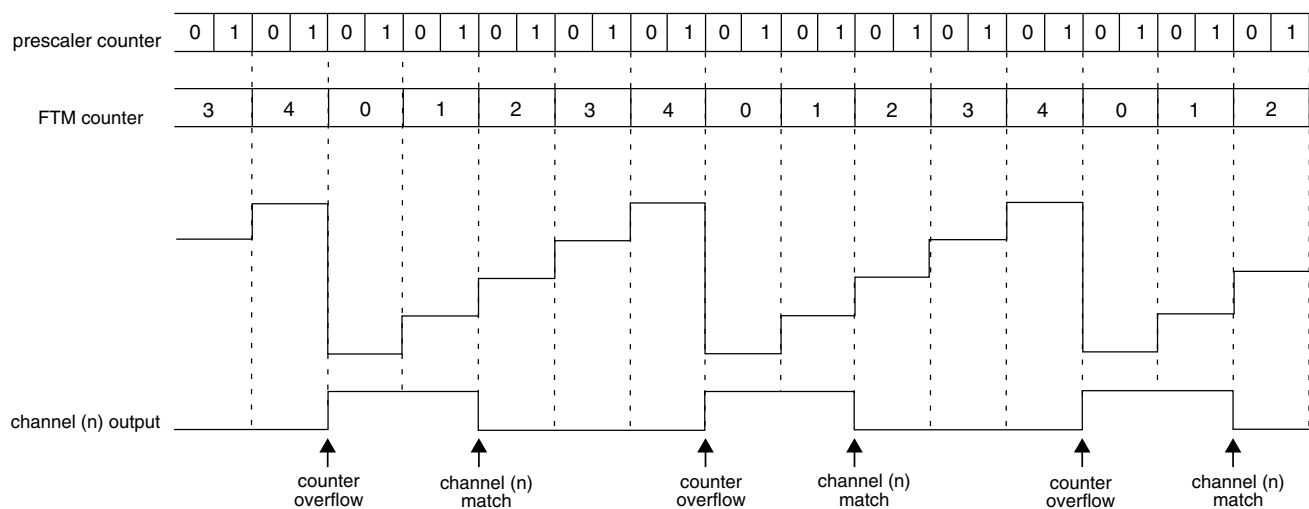
Figure 39-207. Notation used
