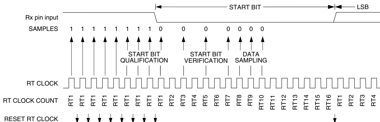
Figure 47-156. Receiver data sampling
