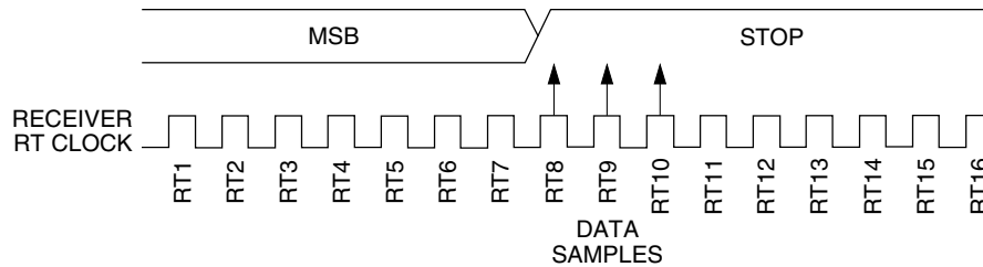
Figure 47-164. Slow data
