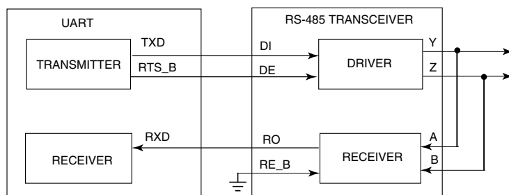
Figure 47-181. Transceiver driver enable using RTS
