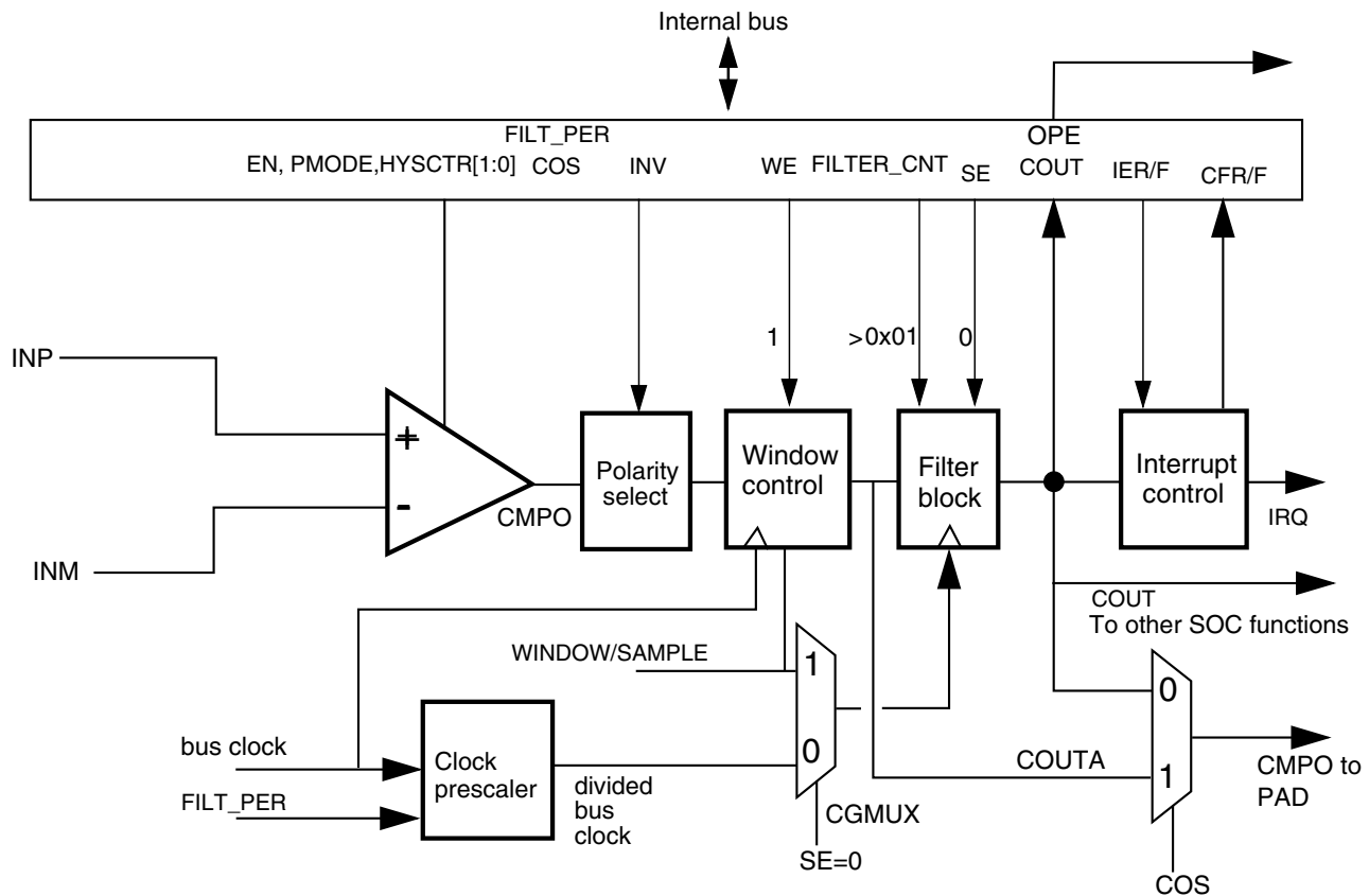
Figure 35-29. Windowed/Filtered mode
