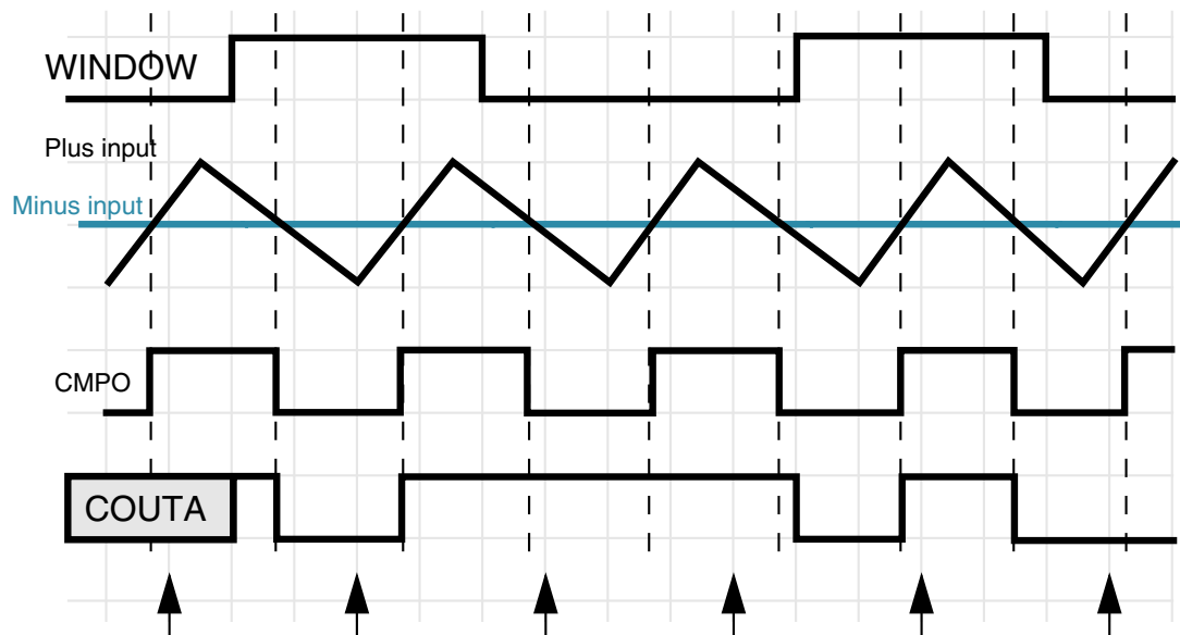
Figure 35-26. Windowed mode operation
