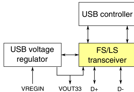
Figure 3-46. USB FS/LS Subsystem Overview
