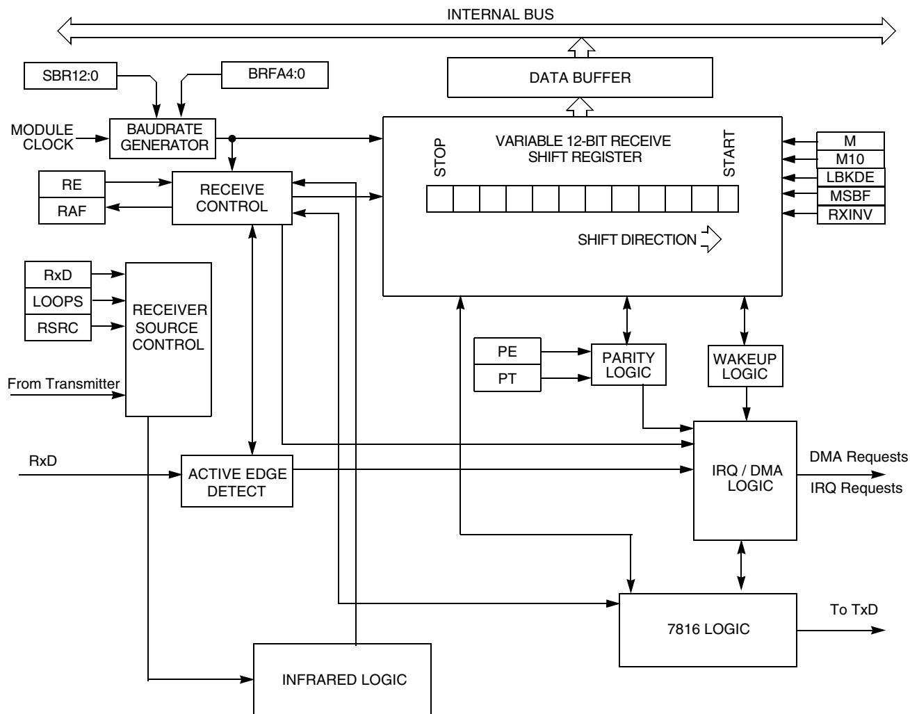
Figure 47-155. UART receiver block diagram
