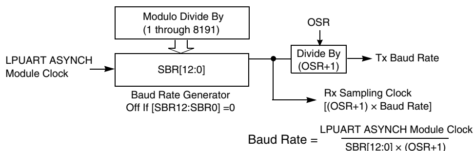
Figure 48-15. LPUART baud rate generation
