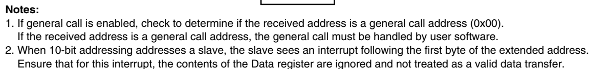
Figure 46-42. Typical I2C interrupt routine
