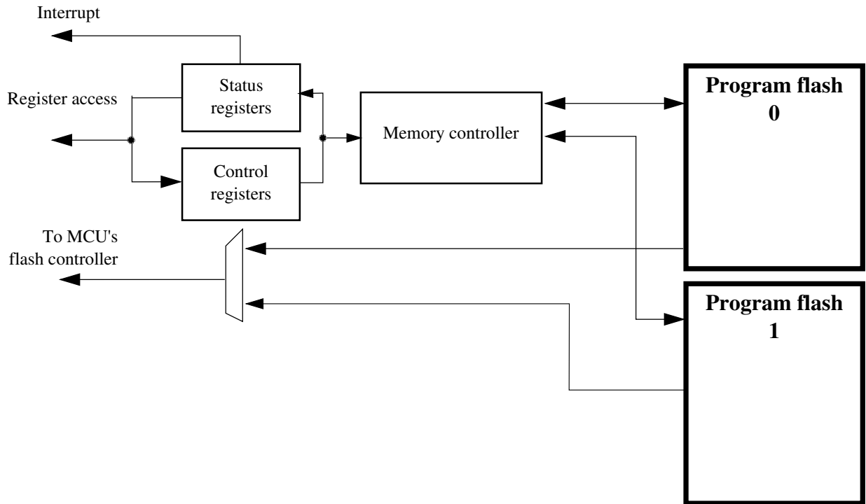
Figure 29-1. Flash Block Diagram
