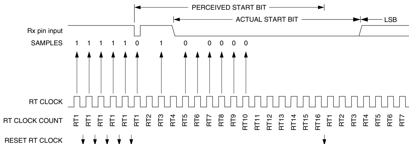
Figure 47-158. Start bit search example 2 ( C7816[ISO\_7816E] = 0 )
