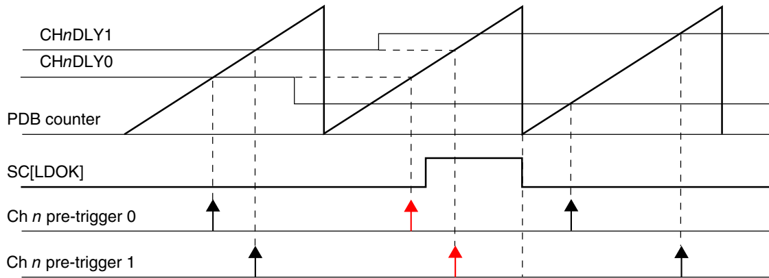
Figure 38-56. Registers update with SC[LDMOD] = x1
