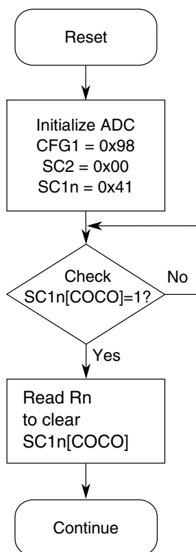
Figure 34-94. Initialization flowchart example
