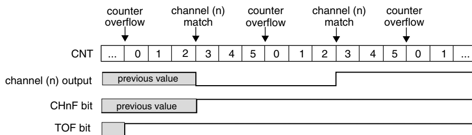
Figure 39-220. Example of the Output Compare mode when the match toggles the channel output
