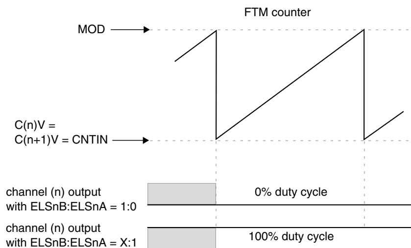
Figure 39-237. Channel (n) output if (C(n)V = C(n+1)V = CNTIN)
