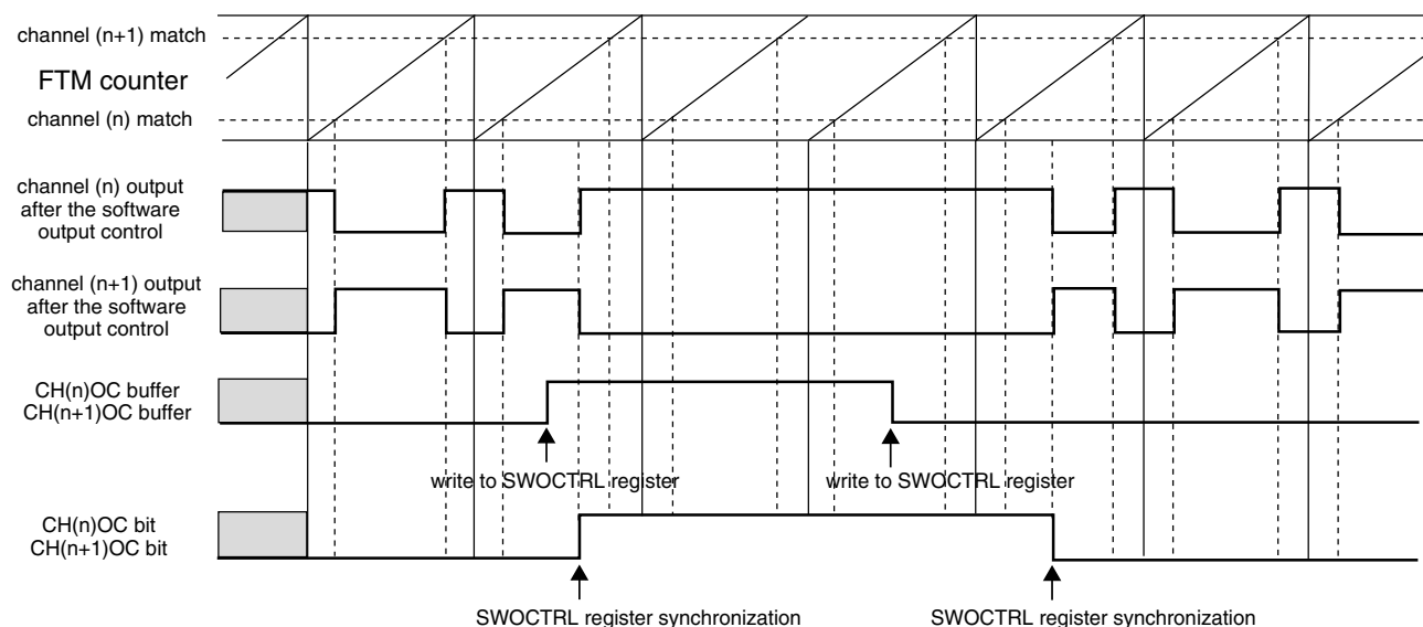
Figure 39-269. Example of software output control in Combine and Complementary mode
