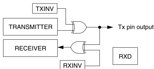
Figure 47-177. Loop operation ( C1[LOOPS] = 1 , C1[RSRC] = 0 )
