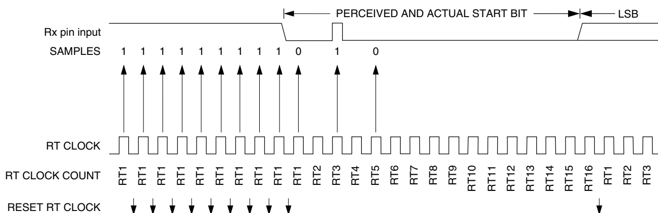
Figure 47-160. Start bit search example 4 (C7816[ISO_7816E] = 0)
