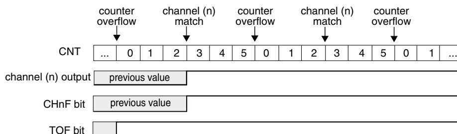
Figure 39-222. Example of the Output Compare mode when the match sets the channel output
