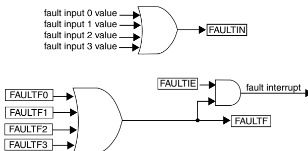
Figure 39-276. FAULTF and FAULTIN bits and fault interrupt
