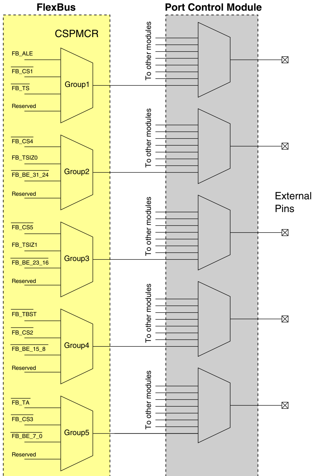
Figure 3-27. FlexBus control signal multiplexing
