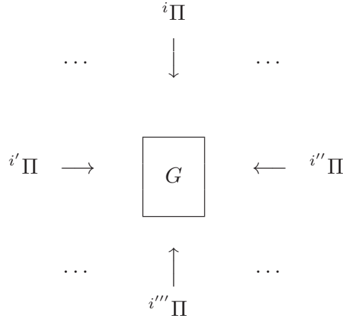
Fig. 1.2: Different arithmetic holomorphic structures on a single coric G
