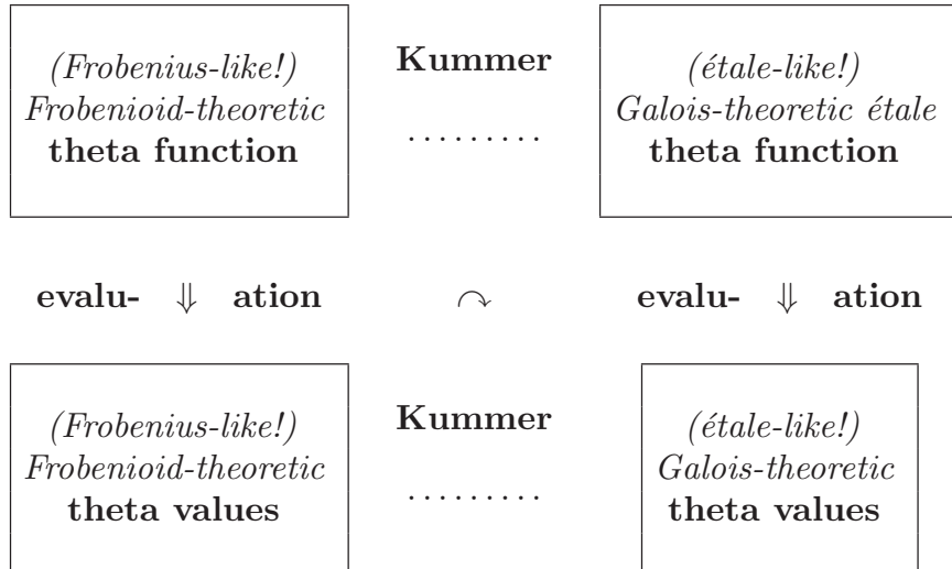
Fig. I.1: The Kummer theory surrounding Hodge-Arakelov-theoretic evaluation
