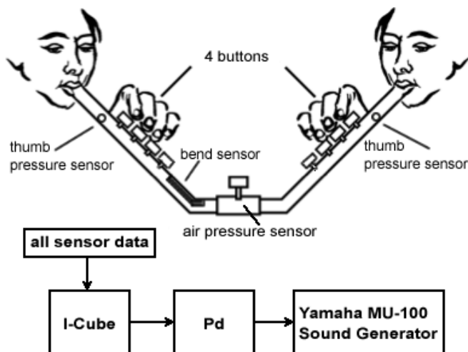
Figure 2: Block diagram of the Tooka.
