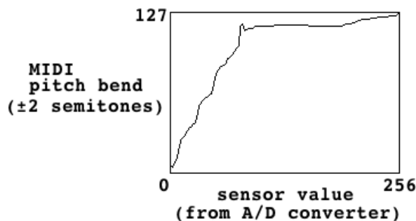
Figure 4: Mapping function to adjust pitch bend
